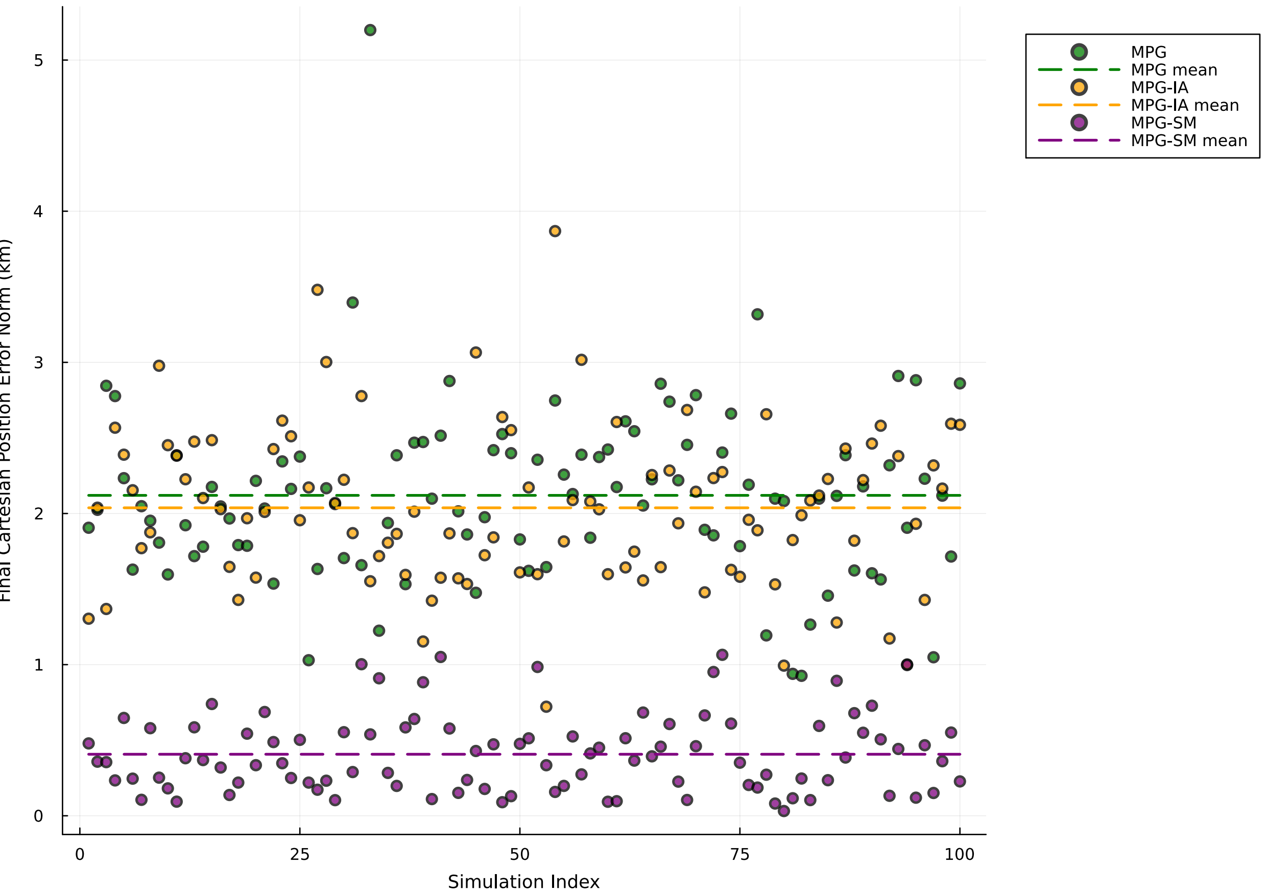
Final Cartesian Position Error Norm (No Open Loop)
