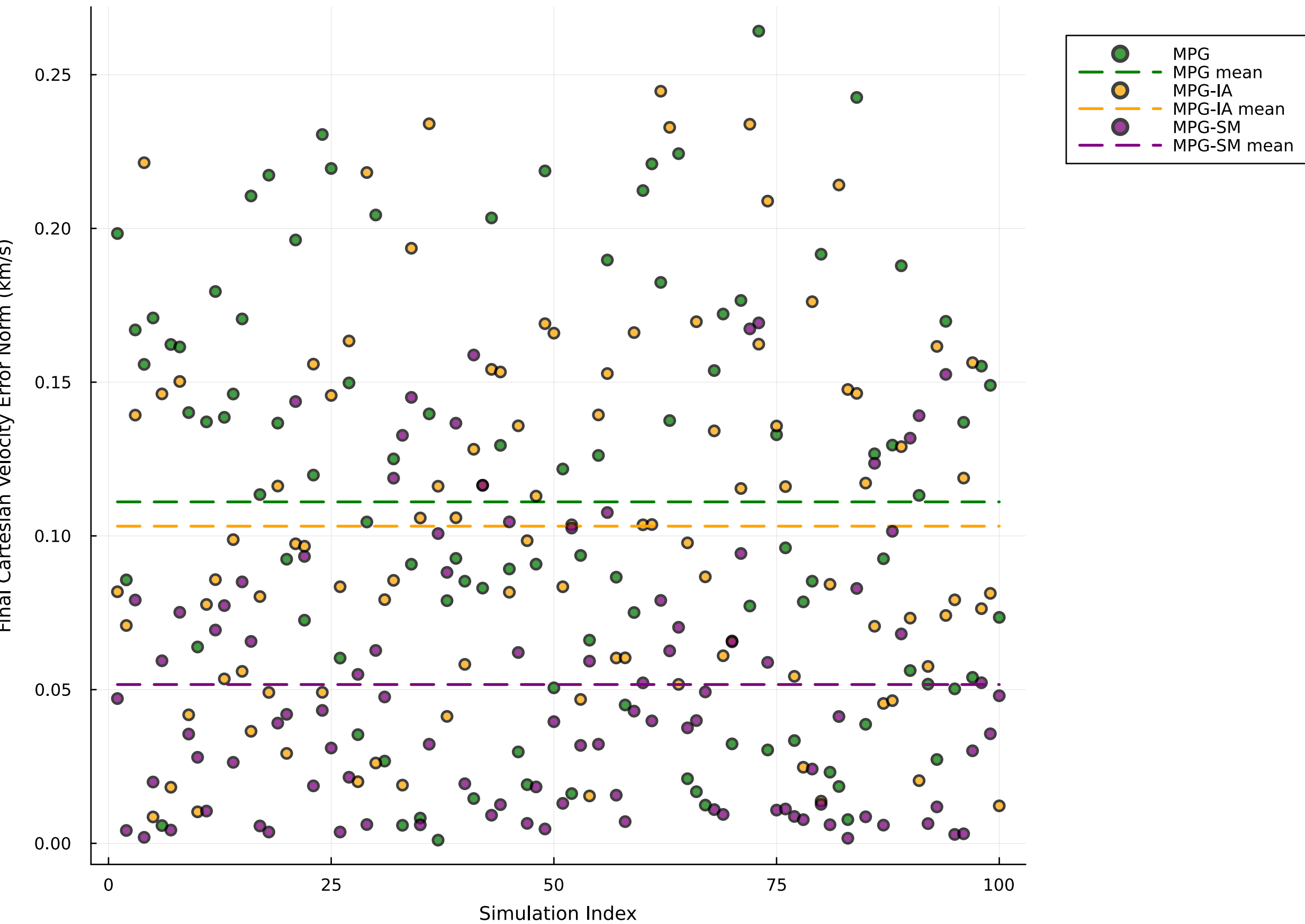
Final Cartesian Velocity Error Norm (No Open Loop)
