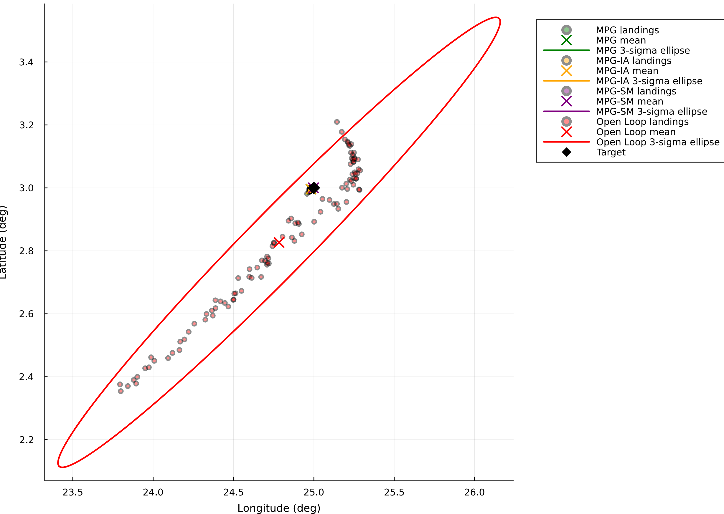
Monte Carlo Simulations: Final Landing Locations With 3-Sigma Ellipses
