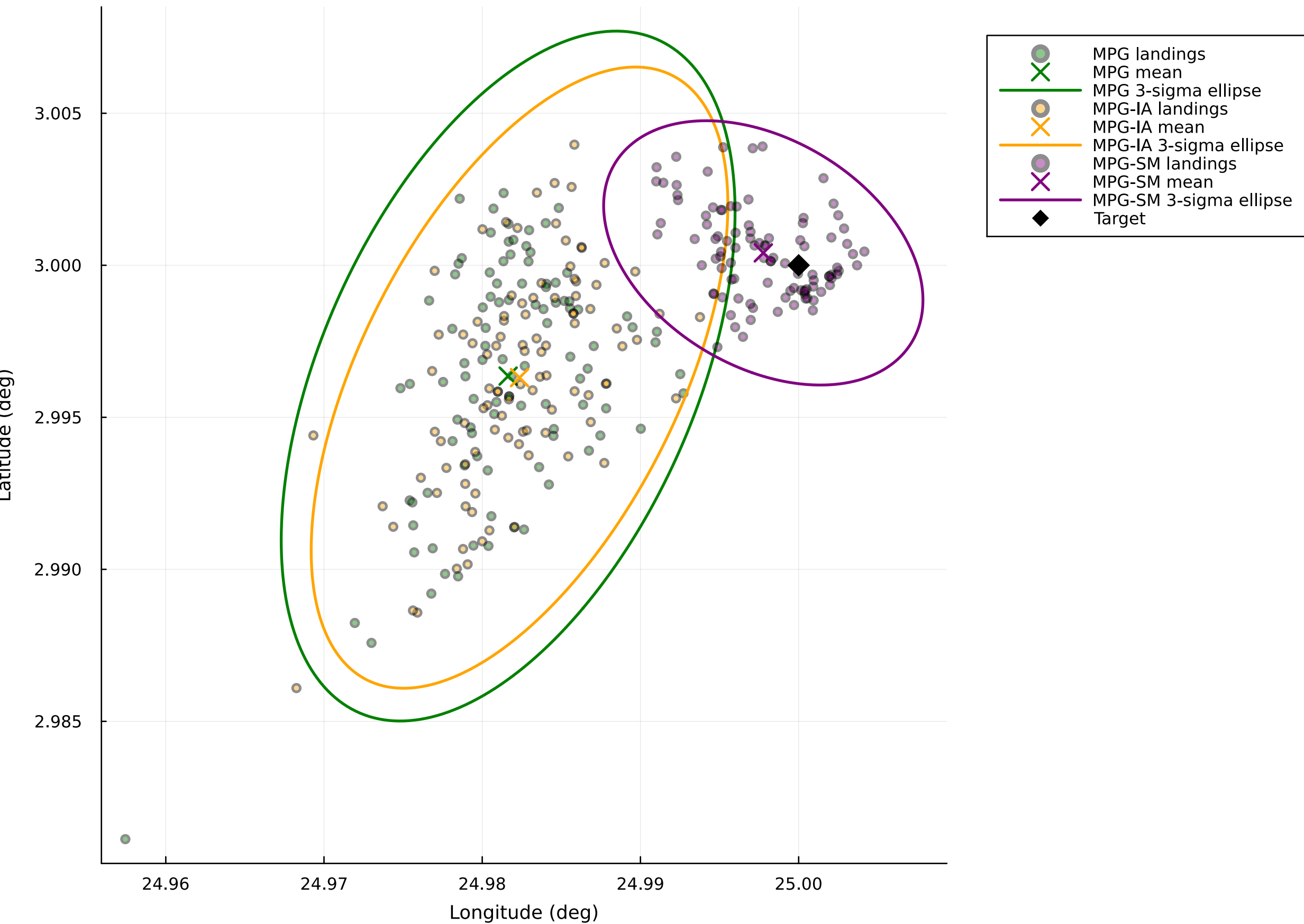
Monte Carlo Simulations: Final Landing Locations With 3-Sigma Ellipses (Without Open Loop)
