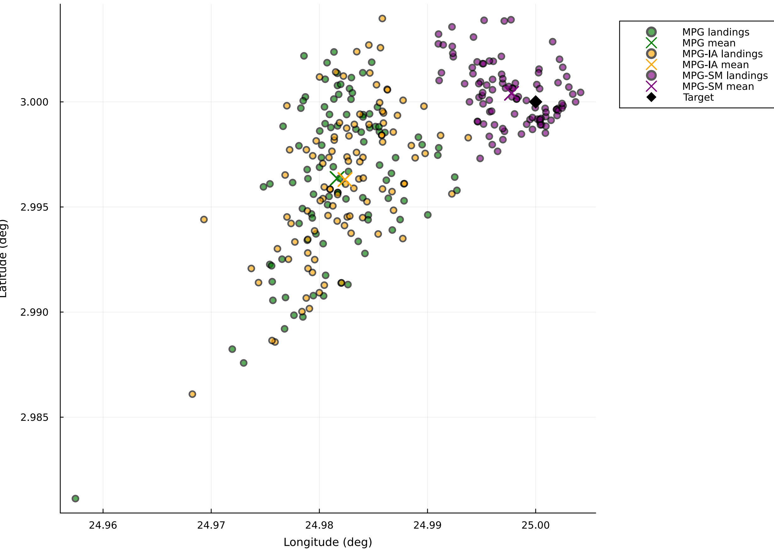
Monte Carlo Simulations: Final Landing Locations (Without Open Loop)
