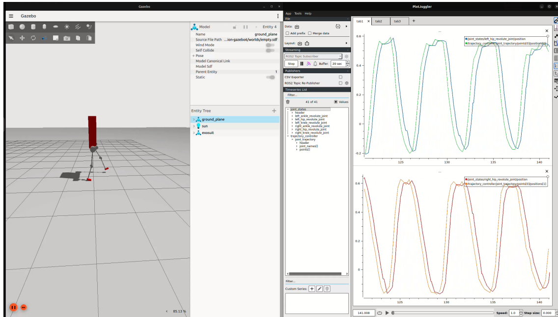
Image 5.5: Gazebo - PlotJuggler Hips Visualization
