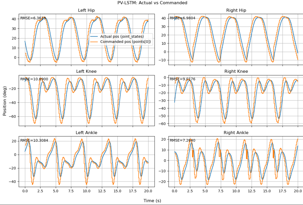
Figure 5.5. joint_states vs commanded_joint_positions for PV LSTM Model
