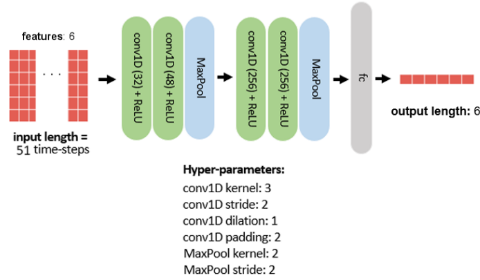
Figure 3.13. Architecture of the CNN model. The timestamp-based and phase variable based variants share this structure and differ only in the number of network inputs.
