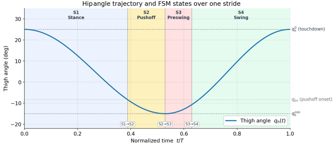
Figure 3.6. Sagittal hip (thigh) angle over one normalized stride, together with the four states of the Finite State Machine.
