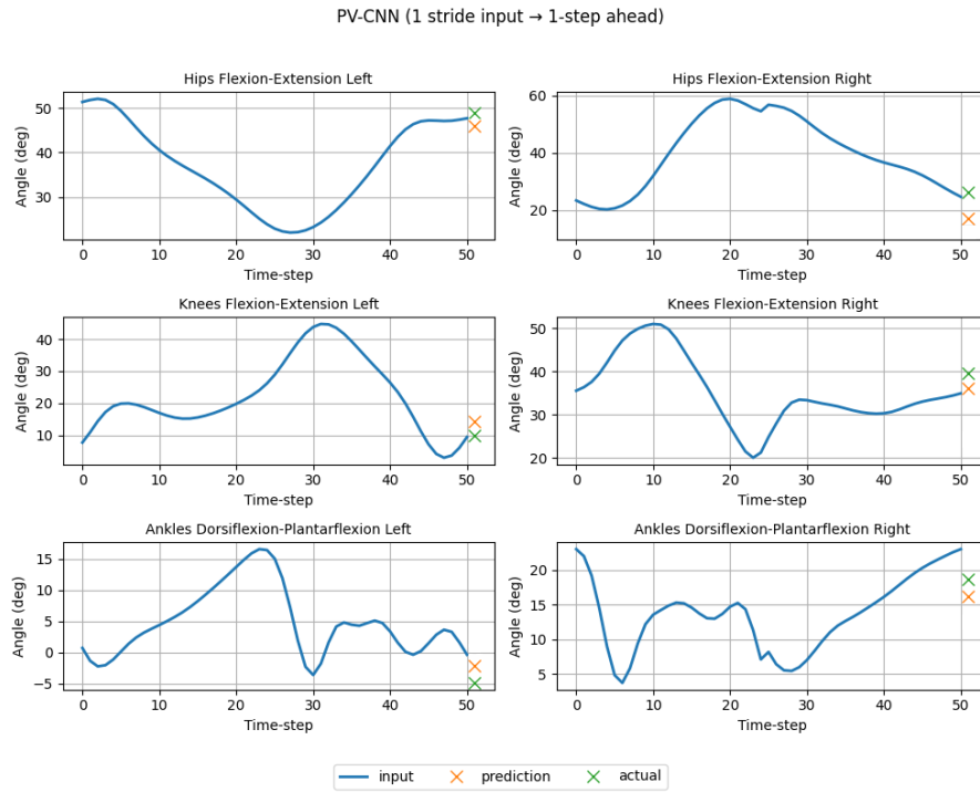
Figure 4.4. PV-CNN: one-stride input and one step ahead prediction.
