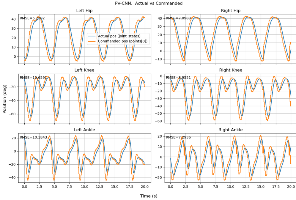
Figure 5.6. joint_states vs commanded_joint_positions for PV CNN Model
