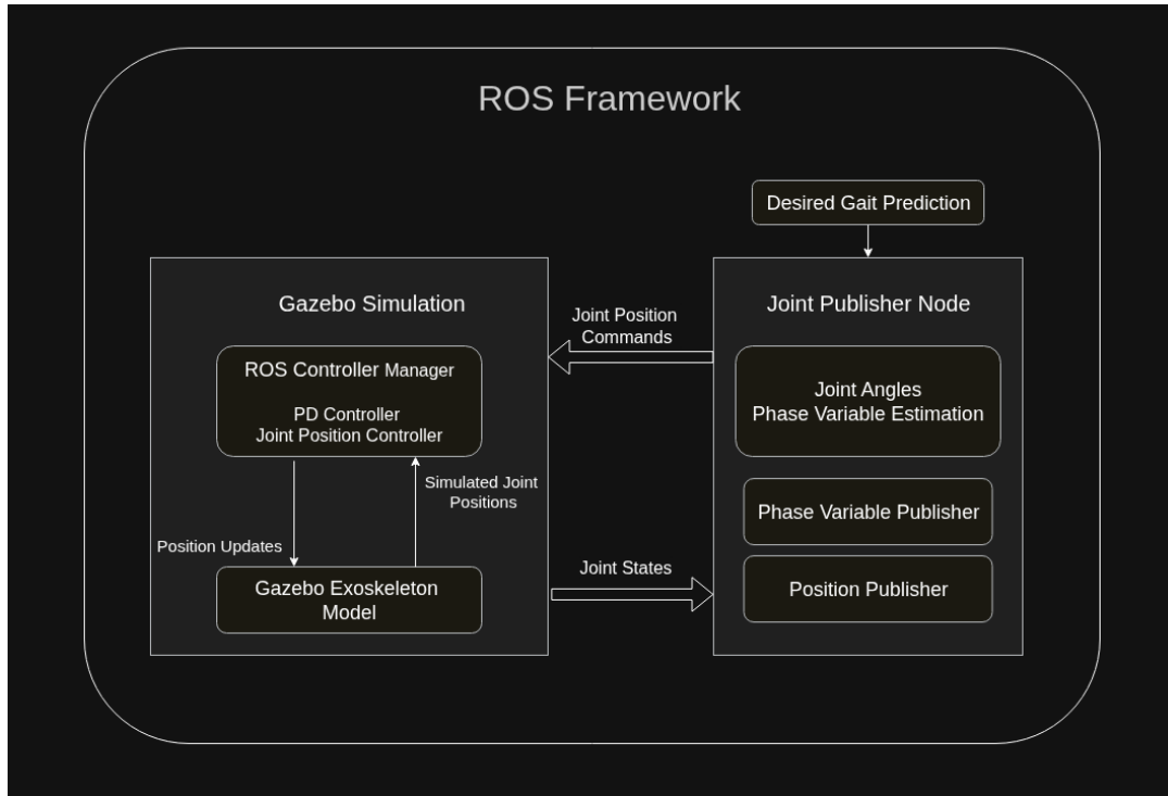
Figure 5.1. The overall simulation architecture.
