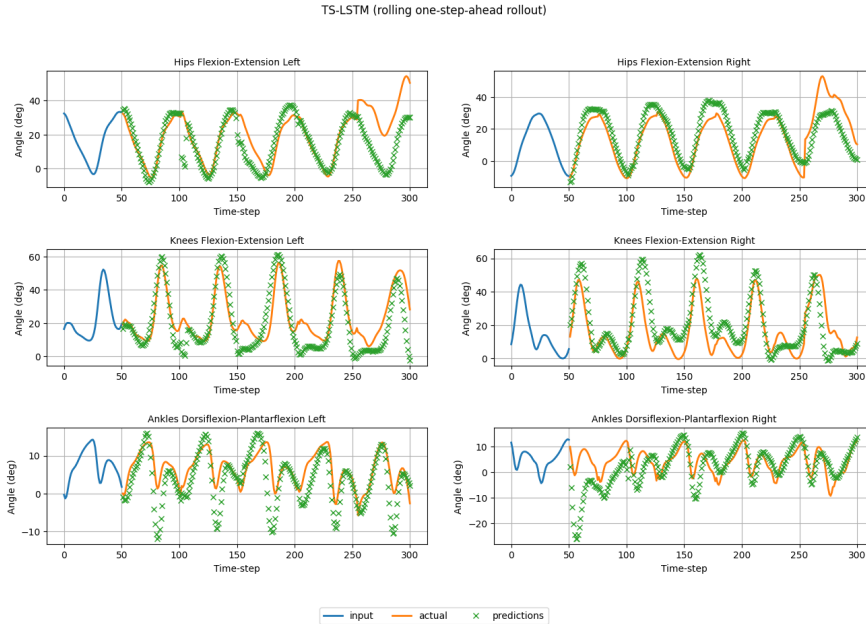
Figure 4.6. TS-LSTM rolling one-step-ahead rollout over multiple strides.
