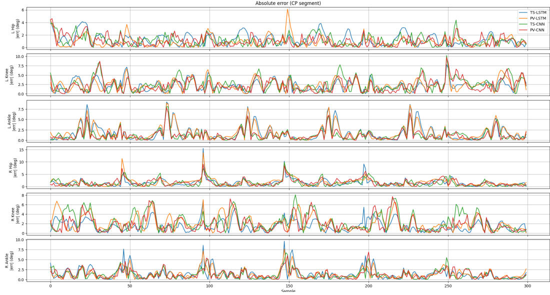
Figure 4.10. Absolute error |e(t)| on the CP segment for all four models.
