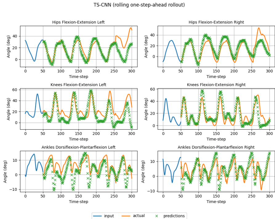
Figure 4.8. TS-CNN rolling one-step-ahead rollout over multiple strides.
