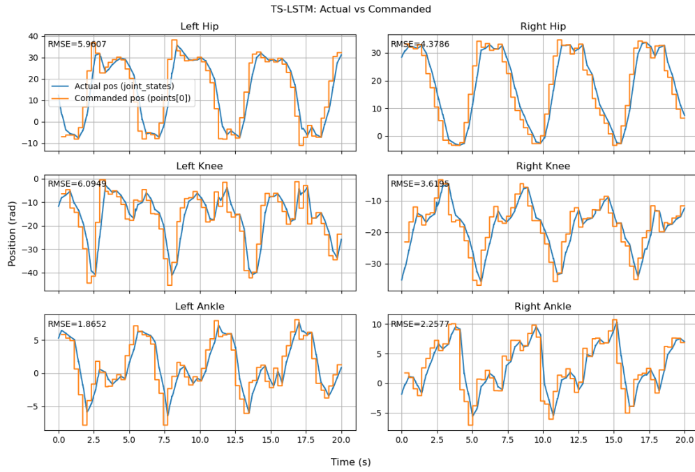
Figure 5.3. joint_states vs commanded_joint_positions for TS LSTM Model
