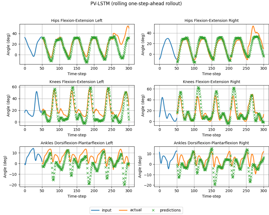
Figure 4.7. PV-LSTM rolling one-step-ahead rollout over multiple strides.
