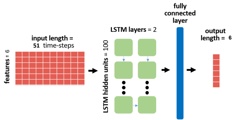
Figure 3.12. Architecture of the LSTM model. The timestamp-based and phase variable based variants share this structure and differ only in the number of network inputs.
