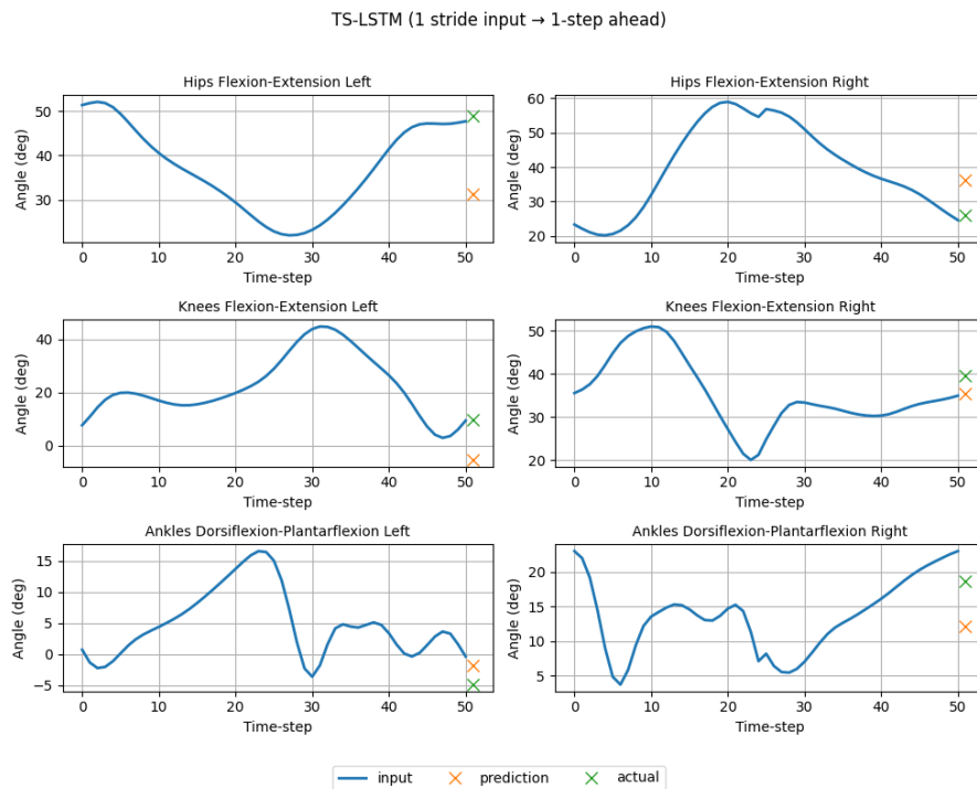
Figure 4.1. TS-LSTM: one-stride input and one step ahead prediction.
