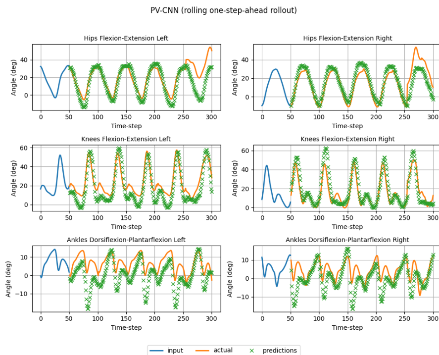
Figure 4.9. PV-CNN rolling one-step-ahead rollout over multiple strides.
