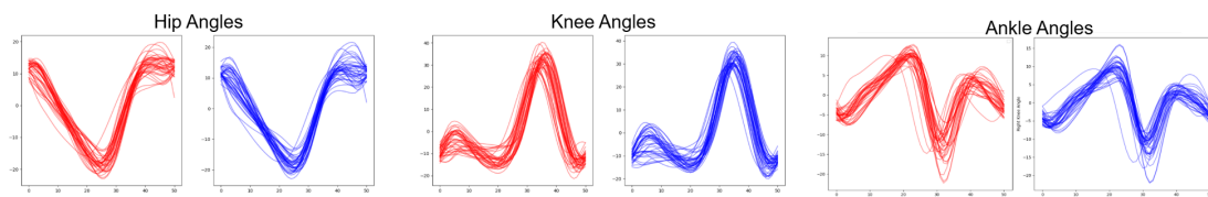
Figure 3.4. TD GAIT cycle over 40 steps on the sagittal plane (Red: left joint angles and Blue: right joint angles)
