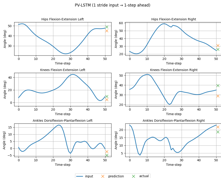
Figure 4.2. PV-LSTM: one-stride input and one step ahead prediction.
