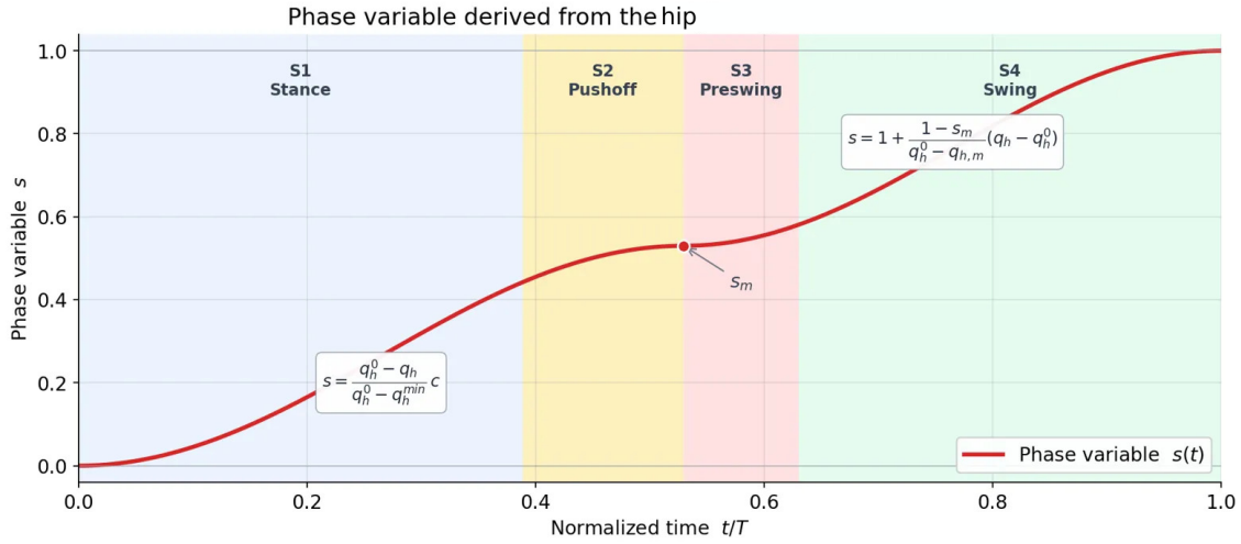
Figure 3.7. Phase variable s obtained from the hip trajectory of Figure 3.6. The stance and pushoff branch (Equation 3.1) is active up to s_m , after which the preswing and swing branch (Equation 3.2) drives s to 1 at the next touchdown. The two branches are joined at the minimum hip angle, producing a continuous and monotonic phase signal.
