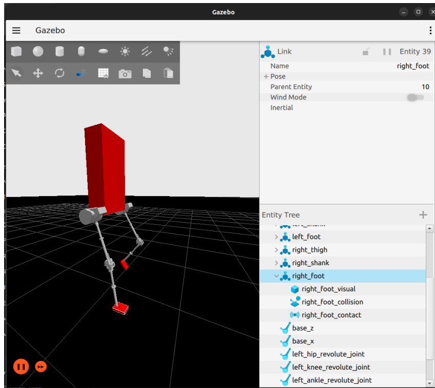
Image 5.4: Screenshot showing feet of the Gazebo model and foot contacts on Entity Tree.
