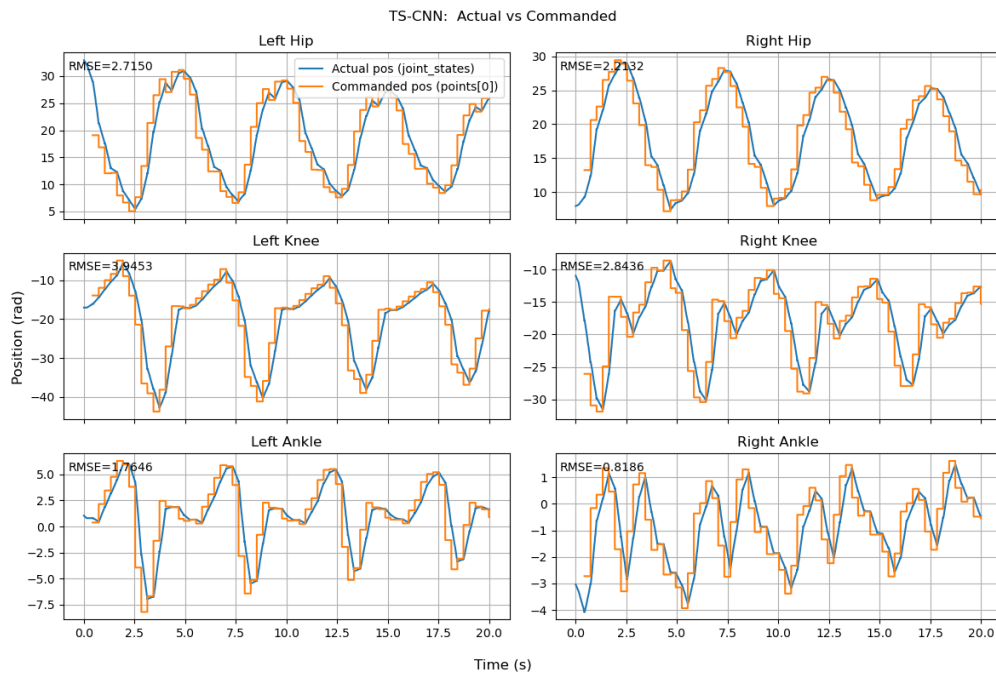
Figure 5.4. joint_states vs commanded_joint_positions for TS CNN Model
