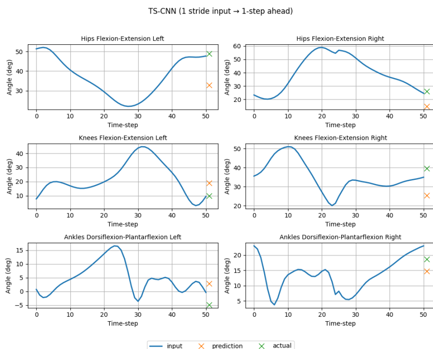
Figure 4.3. TS-CNN: one-stride input and one step ahead prediction.
