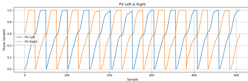
Figure 3.10. Phase Variable Signal on one individual over multiple steps
