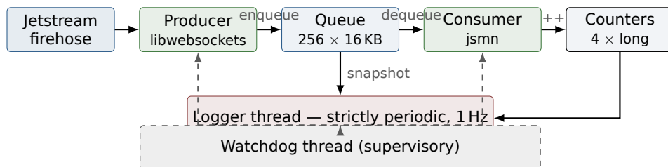
Figure 1: Data flow. The producer and the logger touch the queue; the consumer and the logger touch the counters; the logger is the only thread performing I/O; the watchdog only observes.
