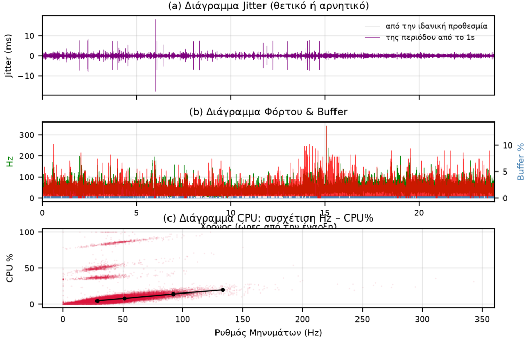
Figure 2: The three required plots over the full 24 hours. (a) Jitter : deviation from the absolute deadline (grey, \geq 0 by construction) and the signed deviation of each one-second period from the ideal (dark). (b) Load and buffer : message rate vs. buffer occupancy. (c) CPU : the correlation of message rate (abscissa) with CPU utilisation, with the median of each rate band in black.
