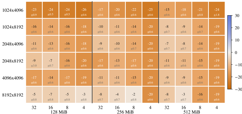
energy saved by a second clock domain (%), vs the measured overlap at the tightest-SLA clock. \pm is a Monte-Carlo upper bound (see caption)
