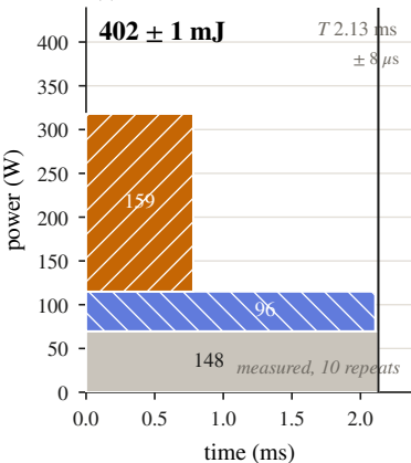
(a) baseline: one domain, 1200 MHz
