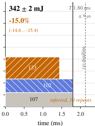
(b) two domains, 510 / 1410 MHz
