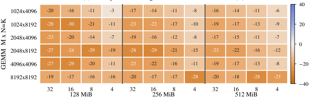
(a) FREE: pick a better single clock, vs what the GPU chose (%)
