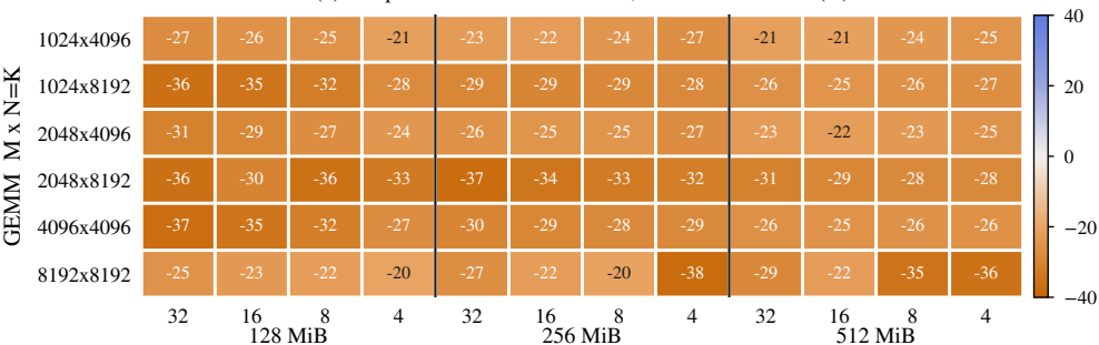
(b) that plus a second clock domain, vs the same default (%)
