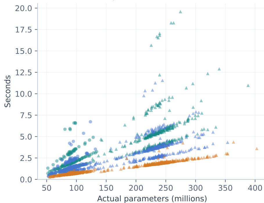
Time to first token 2,000 valid labels
