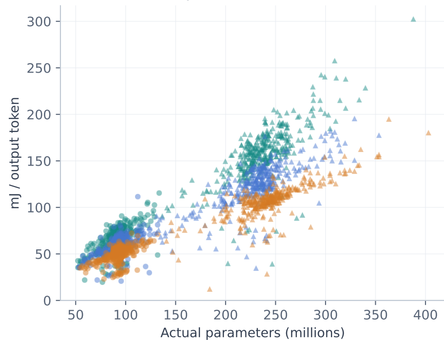
Dynamic energy per token 2,000 valid labels
