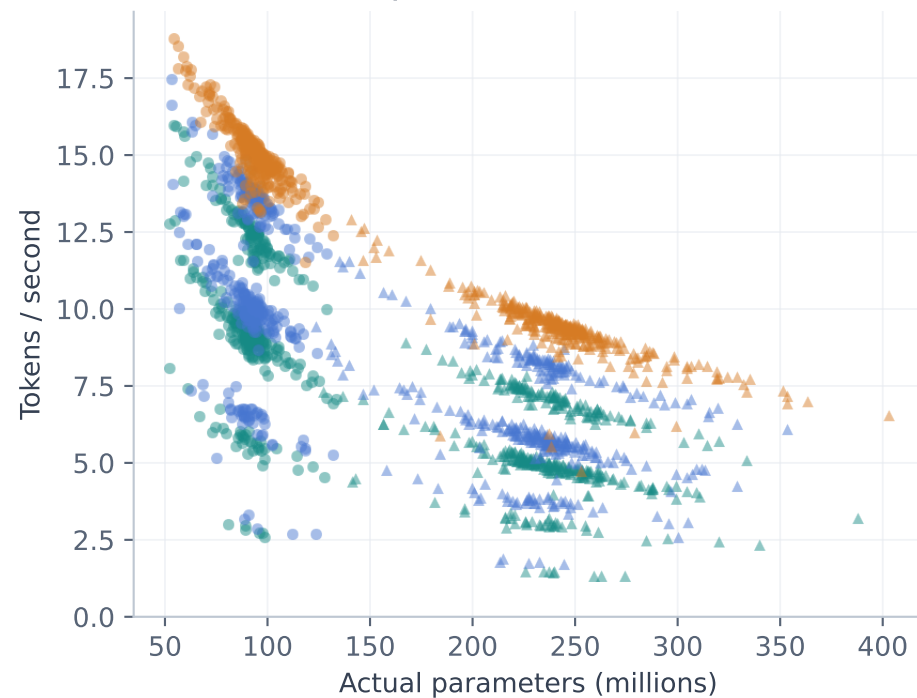
Decode throughput 2,000 valid labels
