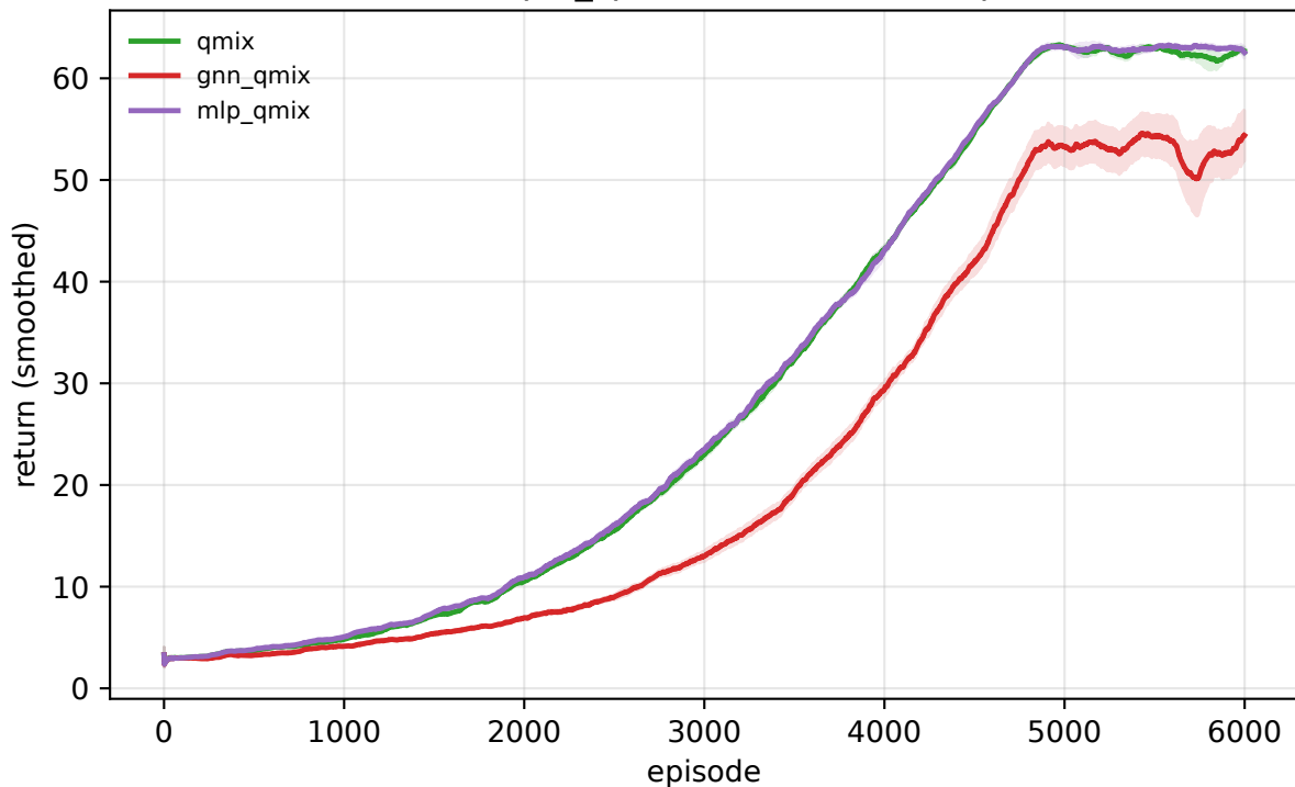
MPE simple_spread N=4 (150k steps)
