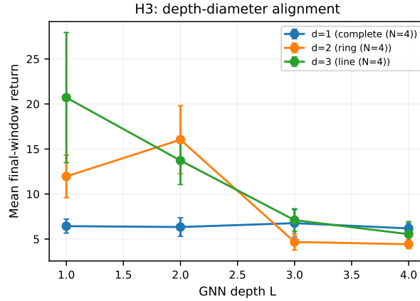
Fig. L2: Phase 4 depth-diameter curves (companion to the heatmap in Section 6.4). Final-window return vs. GCN depth L for each graph diameter d ; the over-depth cliff at L \geq 3 is visible on the structured diameters ( d = 2, 3 ), while the complete graph ( d = 1 ) is flat in L .
