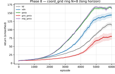
(b) N = 8 (ring).
