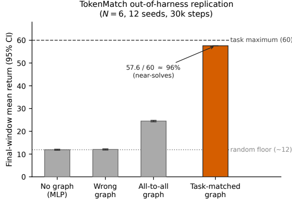
Fig. 14: Out-of-harness replication. Final-window mean return (95% CI, 12 seeds, 30k steps) on TOKENMATCH ( N=6 , K=5 tokens), a non-spatial referential game with no grid, movement, or navigation. The task-matched graph near-solves the task (57.6 of a 60 maximum, \approx 96\% ), completely separating from the wrong-matching graph (12.0) and the no-graph control (11.9), both at the random floor. All-to-all achieves partial routing (24.5; the partner’s token is one of the averaged inputs) but remains far below the task-matched graph. Confirms the structure effect of Figure 11 is not a gridworld artefact.
