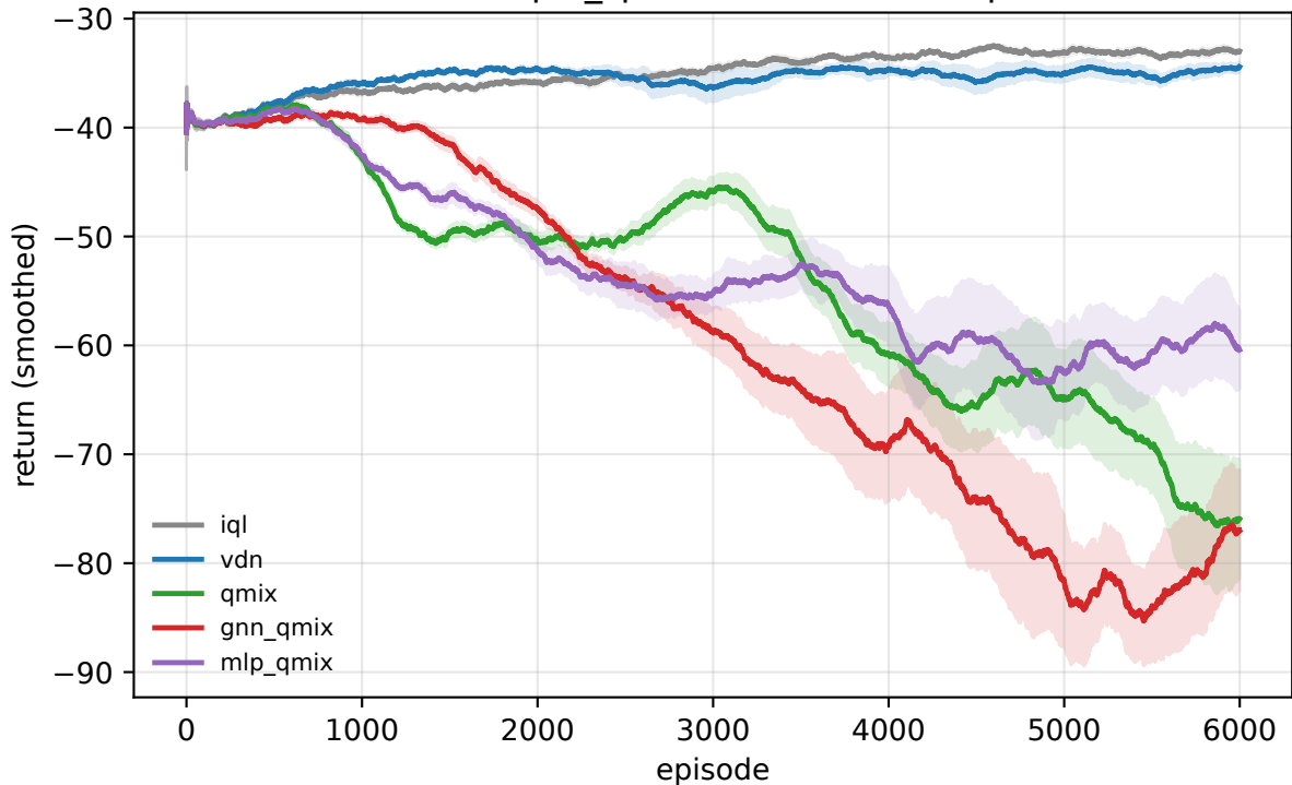
MPE simple_spread N=6 (150k steps)
