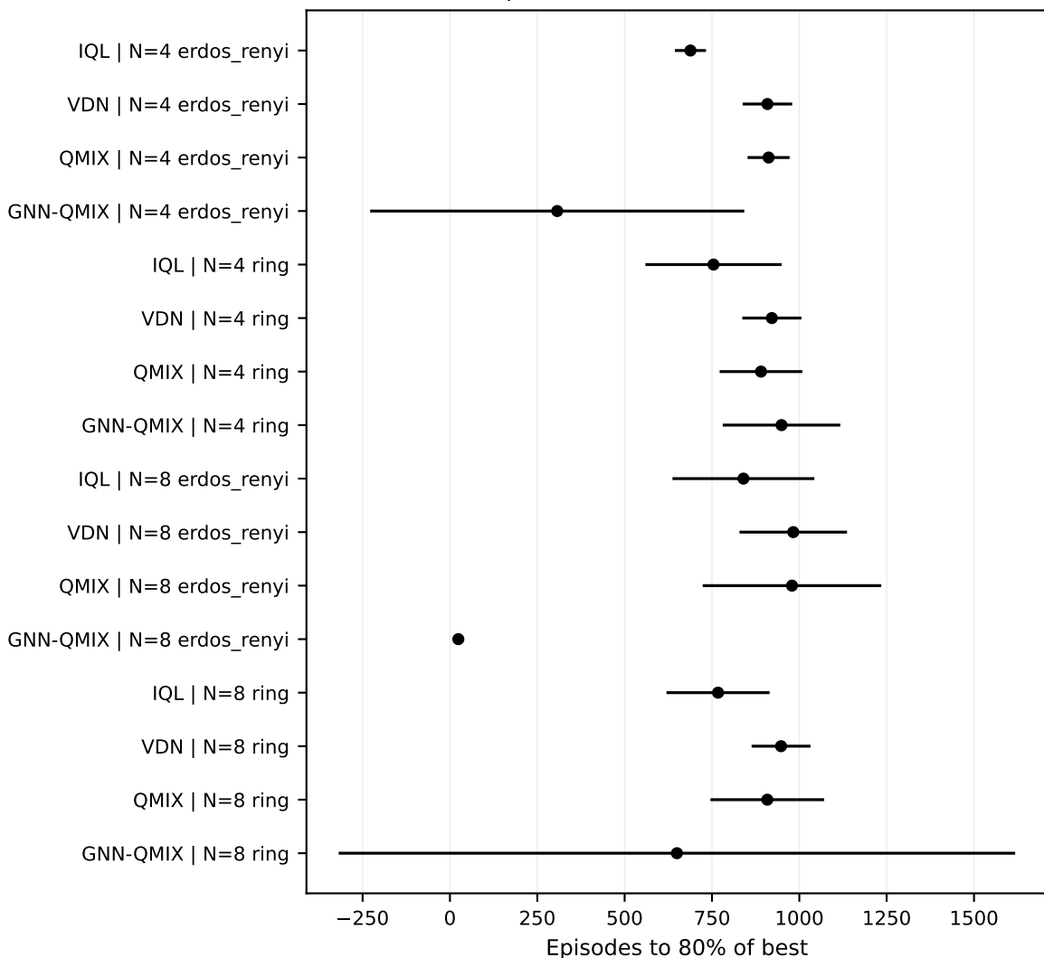
Episodes to 80% of best return
