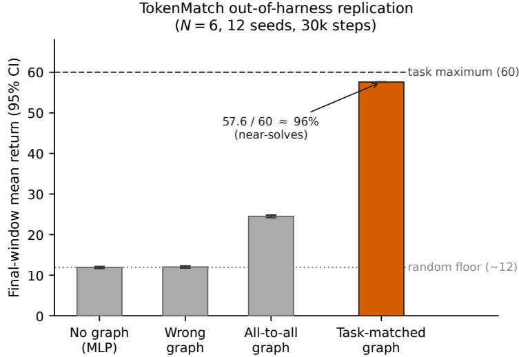
Figure 14: Out-of-harness replication. Final-window mean return (95% CI, 12 seeds, 30k steps) on TOKENMATCH ( N=6 , K=5 tokens), a non-spatial referential game with no grid, movement, or navigation. The task-matched graph near-solves the task (57.6 of a 60 maximum, \approx 96\% ), completely separating from the wrong-matching graph (12.0) and the no-graph control (11.9), both at the random floor. All-to-all achieves partial routing (24.5; the partner’s token is one of the averaged inputs) but remains far below the task-matched graph. Confirms the structure effect of Figure 11 is not a gridworld artefact.
