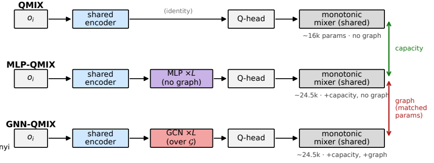
Figure 2: Setup and controlled comparison. (A) COORDGRID: agents act on a grid wired by a tunable coordination graph \mathcal{G} ; the reward is the number of graph edges whose endpoints are co-located, so the graph is the coordination structure. (B) All algorithms share an identical per-agent encoder and monotonic mixer and differ only in the block inserted before the Q-head. QMIX inserts nothing; GNN-QMIX inserts an L -layer GCN over \mathcal{G} ; MLP-QMIX inserts an L -layer MLP of identical parameter count but no graph. GNN-QMIX vs. MLP-QMIX isolates the graph (matched parameters); MLP-QMIX vs. QMIX isolates the capacity .
