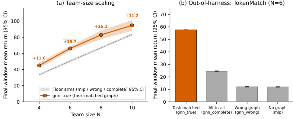
Fig. 12: Left: the advantage holds across team size but is non-monotone. Task-matched gnn_true (solid line) stays above the control floor (shaded band: mlp / wrong / all-to-all 95% CI) at every N \in \{4, 6, 8, 10\} ; the gap over the no-graph floor (labelled) peaks near N=8 rather than growing monotonically. Right: out-of-harness replication on TOKENMATCH (shown standalone, with discussion, as Figure 14 in §7.8). All bars/points are 95% CIs over 12 seeds.
