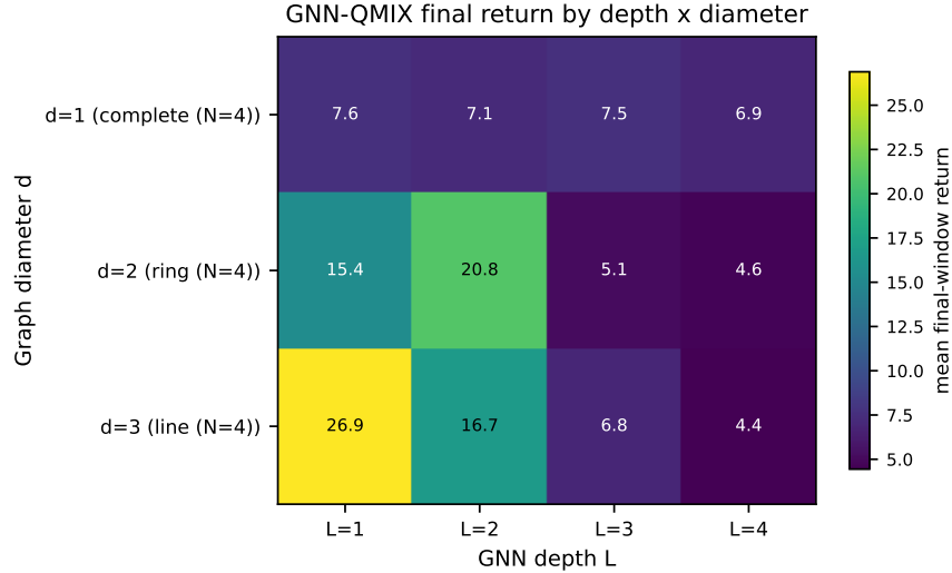
Figure 2: Phase 4: GNN-QMIX final-window mean return as a function of GNN depth L and coordination graph diameter d . Cells along the diagonal correspond to depth–diameter alignment ( L \approx d ), the H3 prediction.
