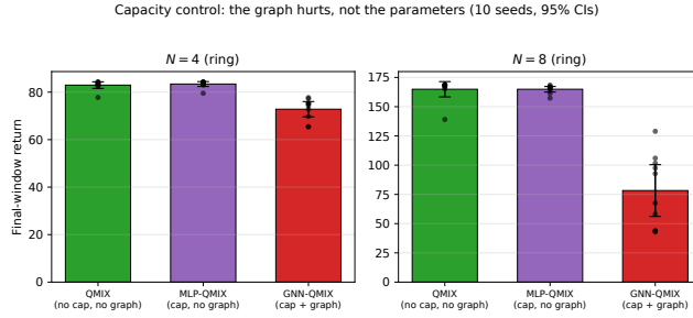
Figure 6: Capacity control on COORDGRID ring . MLP-QMIX (same parameter count as GNN-QMIX, no graph) tracks QMIX, while GNN-QMIX falls far below both at both team sizes: the penalty is the graph aggregation, not the added capacity. Means over 10 seeds; 95% Student- t CIs.
