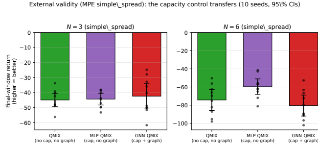
Figure 5: External validity on MPE simple_spread (10 seeds, 95% CIs; less negative is better). At N=6 , MLP-QMIX (matched parameters, no graph) sits above QMIX while GNN-QMIX falls below both: the positive capacity effect and the negative graph effect the decomposition (Table 9) separates.
