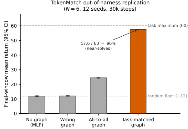
Fig. 14: Out-of-harness replication. Final-window mean return (95% CI, 12 seeds, 30k steps) on TOKENMATCH ( N=6 , K=5 tokens), a non-spatial referential game with no grid, movement, or navigation. The task-matched graph near-solves the task (57.6 of a 60 maximum, \approx 96\% ), completely separating from the wrong-matching graph (12.0) and the no-graph control (11.9), both at the random floor. All-to-all achieves partial routing (24.5; the partner’s token is one of the averaged inputs) but remains far below the task-matched graph. Confirms the structure effect of Figure 11 is not a gridworld artefact.
