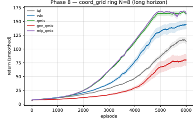
(b) N = 8 (ring).
