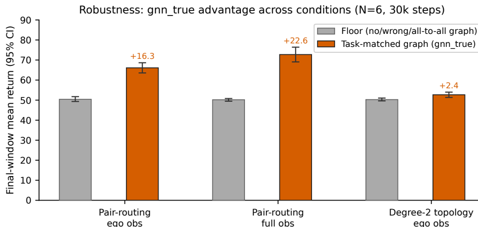
Fig. 13: The advantage is robust across conditions. Task-matched gnn_true (orange) versus the control floor (gray: no/wrong/all-to-all graph), 95% CI over 12 seeds at N=6 (30k steps). The structure advantage holds under ego observations (+16.3) and is larger under full observability (+22.6); at genuine degree-2 topology it survives but shrinks sharply (+2.4), consistent with a fixed mean-aggregator exploiting a neighbourhood-set (centroid) task far less efficiently than single-partner routing.
