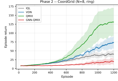
(b) N = 8 , ring.
