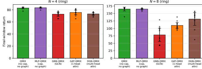
Fig. 9: Second GNN family. Single-head (GAT-QMIX) and multi-head (DGN-QMIX, the DGN/G2ANet operator) graph attention both sit above GNN-QMIX (the fixed GCN), more expressive attention helps within graph methods, but still below the parameter-matched no-graph control MLP-QMIX at both team sizes on Coord-Grid: no unstabilised graph operator recovers a benefit here (cf. Appendix I, where the stabilised GCN reaches parity but still does not exceed the control).
