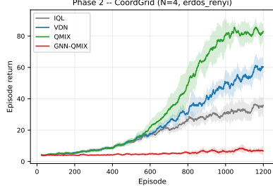
(a) N = 4 , Erdős–Rényi (matched density).
