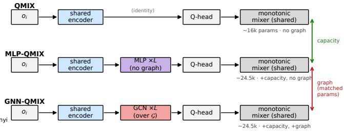
Fig. 2: Setup and controlled comparison. (A) COORDGRID: agents act on a grid wired by a tunable coordination graph G ; the reward is the number of graph edges whose endpoints are co-located, so the graph is the coordination structure. (B) All algorithms share an identical per-agent encoder and monotonic mixer and differ only in the block inserted before the Q-head. QMIX inserts nothing; GNN-QMIX inserts an L -layer GCN over G ; MLP-QMIX inserts an L -layer MLP of identical parameter count but no graph. GNN-QMIX vs. MLP-QMIX isolates the graph (matched parameters); MLP-QMIX vs. QMIX isolates the capacity .
