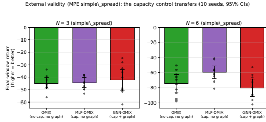
Fig. 5: External validity on MPE simple_spread (10 seeds, 95% CIs; less negative is better). At N=6 , MLP-QMIX (matched parameters, no graph) sits above QMIX while GNN-QMIX falls below both: the positive capacity effect and the negative graph effect the decomposition (Table E3) separates.
