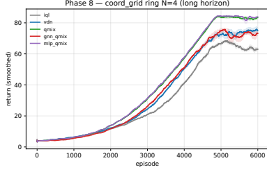
(a) N = 4 (ring).
