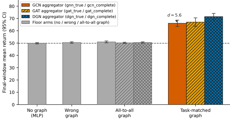
Fig. 11: It is the structure, not the channel. Final-window mean return (95% CI, 12 seeds) on the pair-routing task ( N=6 , ego observations, 30k steps). Only the task-matched graph rises well above the random floor ( \sim 50 ): the no-graph control (mlp) and a density-matched wrong graph sit at the floor, the all-to-all graph (the most communication) one point above it, while the task-matched graph reaches 66–71 depending on the aggregator ( d \approx 5 vs. the floor). Learned attention (GAT, DGN) helps only on the matched graph; over all-to-all it floors like the fixed GCN. The right edges, not more edges, carry the advantage.
