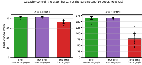
Fig. 7: Capacity control on COORDGRID ring. MLP-QMIX (same parameter count as GNN-QMIX, no graph) tracks QMIX, while GNN-QMIX falls far below both at both team sizes: the penalty is the graph aggregation, not the added capacity. Means over 10 seeds; 95% Student- t CIs.
