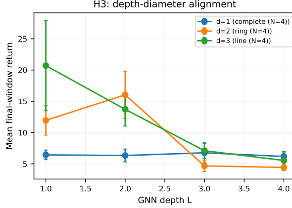
Fig. M2: Phase 4 depth–diameter curves (companion to the heatmap in Section 6.4). Final-window return vs. GCN depth L for each graph diameter d ; the over-depth cliff at L \geq 3 is visible on the structured diameters ( d = 2, 3 ), while the complete graph ( d = 1 ) is flat in L .
