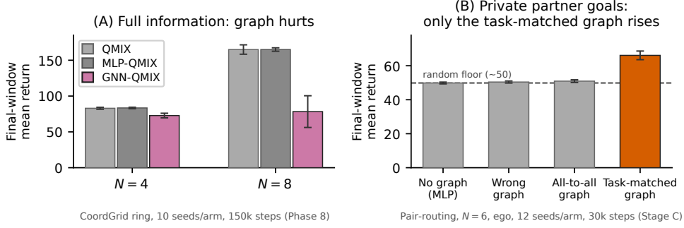
Fig. 1: Both boundary endpoints at a glance. (A) Negative endpoint: on full-information COORDGRID (ring graph) the graph buys nothing—and the standard unstabilised GNN-QMIX (capacity-matched, +graph) shown here falls below both QMIX (no graph) and the parameter-matched MLP-QMIX (no graph) control at N=4 and N=8 (10 seeds, 150k steps; 95% CI). That deficit is an optimisation pathology: a stabilised GCN recovers to parity with the controls (Appendix I), still without any benefit. (B) Positive endpoint: on the pair-routing task, where each agent must act on a partner’s privately held goal, only the task-matched graph rises well above the random floor ( \approx 50 ); a density-matched wrong graph and the all-to-all graph stay at or within a point of the floor (12 seeds, 30k steps; 95% CI). The same stabilised graph-conditioned architecture is thus inert under full information (parity, panel A via Appendix I) yet a large asset when the task requires routing information the receiver cannot otherwise observe (panel B)—the discriminator is the task’s information structure, not the architecture.
