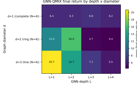
Fig. 6: Phase 4: GNN-QMIX final-window mean return as a function of GNN depth L and coordination graph diameter d . Cells along the diagonal correspond to depth–diameter alignment ( L \approx d ), the H3 prediction. Outcome: H3 is not confirmed at the family level (1/3 diameters pass); on the structured diameters ( d = 2, 3 ) the two rightmost columns ( L = 3, 4 ) collapse—an over-depth cliff—while the complete graph ( d = 1 ) is flat in L .
