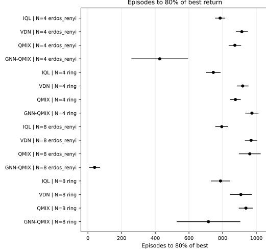
Fig. 3: Phase 2 forest plot: episodes to 80% of each run’s own final-window return, per algorithm \times condition (the panel-invariant self-threshold metric of Section 5.3). Lower is better. Bars are 95% Student- t CIs across seeds. Per-condition returns and the H1/H2 hypothesis tests are in Appendix L (Tables L12, L14, L15).
