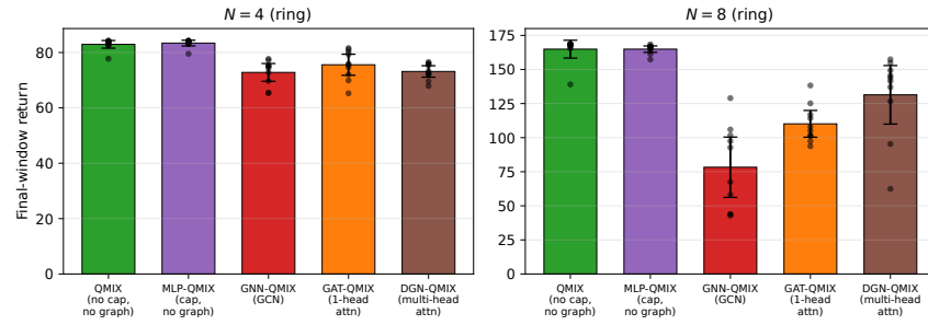
Fig. 8. Second GNN family. Single-head (GAT-QMIX) and multi-head (DGN-QMIX, the DGN/G2ANet operator) graph attention both sit above GNN-QMIX (the fixed GCN), more expressive attention helps within graph methods, but still below the parameter-matched no-graph control MLP-QMIX at both team sizes on CoordGrid: the graph in its strongest form remains a net liability.
