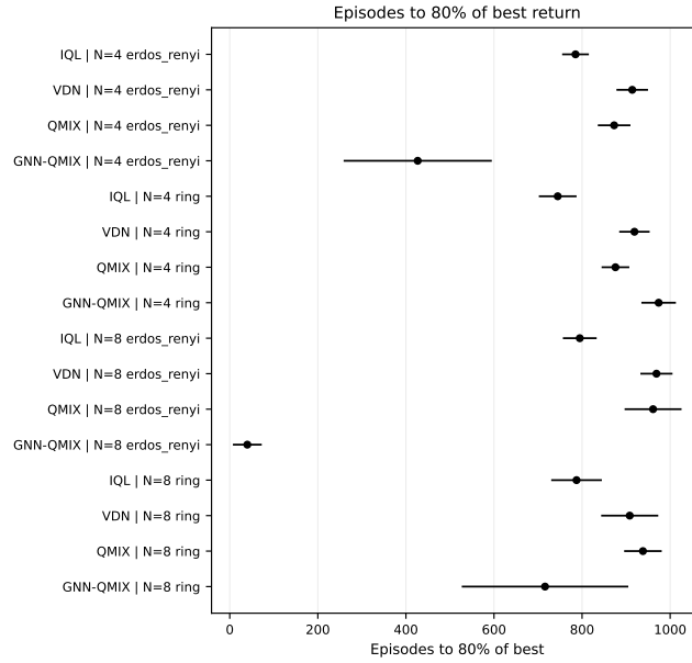
Fig. 2. Phase 2 forest plot: episodes to 80% of best final-window return per algorithm \times condition. Lower is better. Bars are 95% Student- t CIs across seeds. Per-condition returns and the H1/H2 hypothesis tests are in Appendix J (Tables 13, 15, 16).
