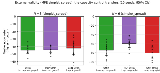
Fig. 4. External validity on MPE simple_spread (10 seeds, 95% CIs; less negative is better). At N=6 , MLP-QMIX (matched parameters, no graph) sits above QMIX while GNN-QMIX falls below both: the positive capacity effect and the negative graph effect the decomposition (Table 6) separates.
