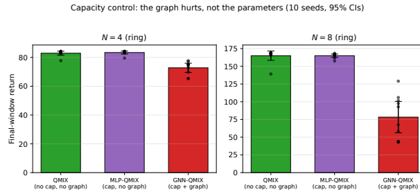
Fig. 6. Capacity control on COORDGRID ring. MLP-QMIX (same parameter count as GNN-QMIX, no graph) tracks QMIX, while GNN-QMIX falls far below both at both team sizes: the penalty is the graph aggregation, not the added capacity. Means over 10 seeds; 95% Student- t CIs.
