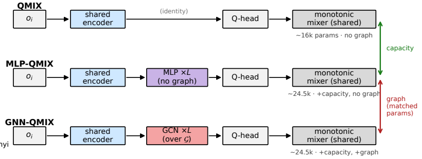
Fig. 1. Setup and controlled comparison. (A) COORDGRID: agents act on a grid wired by a tunable coordination graph \mathcal{G} ; the reward is the number of graph edges whose endpoints are co-located, so the graph is the coordination structure. (B) All algorithms share an identical per-agent encoder and monotonic mixer and differ only in the block inserted before the Q-head. QMIX inserts nothing; GNN-QMIX inserts an L -layer GCN over \mathcal{G} ; MLP-QMIX inserts an L -layer MLP of identical parameter count but no graph. GNN-QMIX vs. MLP-QMIX isolates the graph (matched parameters); MLP-QMIX vs. QMIX isolates the capacity .
