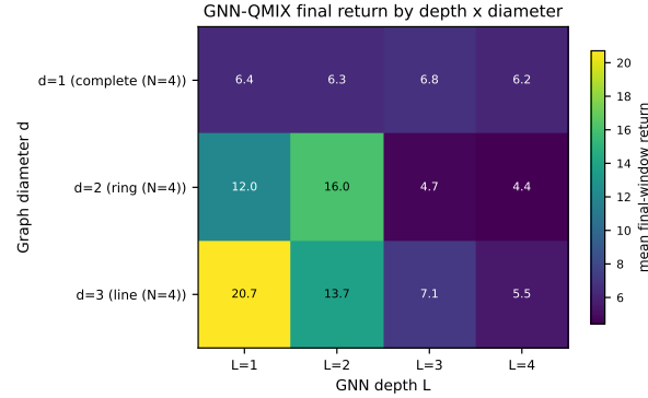
Fig. 5. Phase 4: GNN-QMIX final-window mean return as a function of GNN depth L and coordination graph diameter d . Cells along the diagonal correspond to depth–diameter alignment ( L \approx d ), the H3 prediction.
