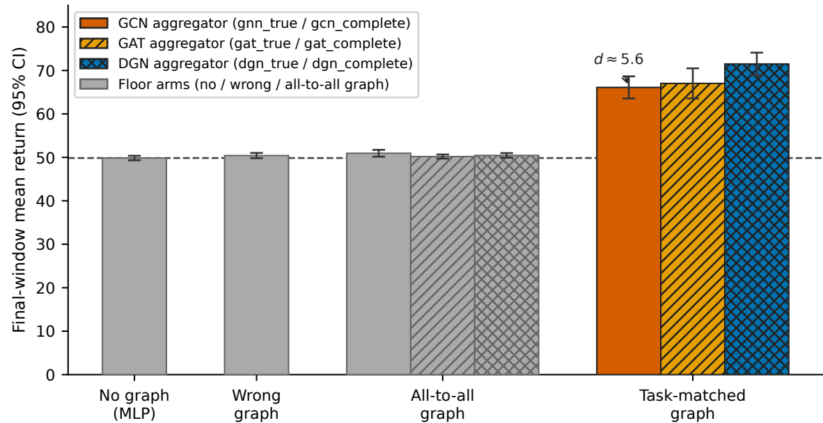
Fig. 10. It is the structure, not the channel. Final-window mean return (95% CI, 12 seeds) on the pair-routing task ( N=6 , ego observations, 30k steps). Only the task-matched graph rises above the random floor ( \sim 50 ): the no-graph control (mlp), a density-matched wrong graph, and the all-to-all graph (the most communication) all sit at the floor, while the task-matched graph reaches 66–71 depending on the aggregator ( d \approx 5 vs. the floor). Learned attention (GAT, DGN) helps only on the matched graph; over all-to-all it floors like the fixed GCN—more communication does not help, the right communication does.
