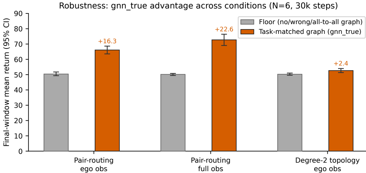
Fig. 12. The advantage is robust across conditions. Task-matched gnn_true (orange) versus the control floor (gray: no/wrong/all-to-all graph), 95% CI over 12 seeds at N=6 (30k steps). The structure advantage holds under ego observations (+16.3) and is larger under full observability (+22.6); at genuine degree-2 topology it survives but shrinks sharply (+2.4), consistent with a fixed mean-aggregator exploiting a neighbourhood-set (centroid) task far less efficiently than single-partner routing.
