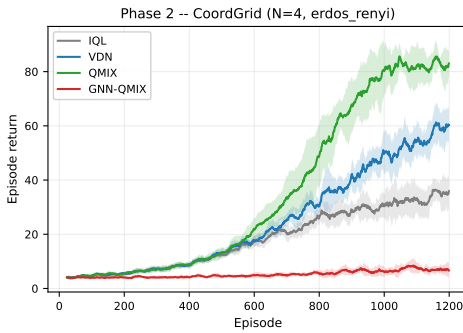
(a) N = 4 , Erdős-Rényi (matched density).
