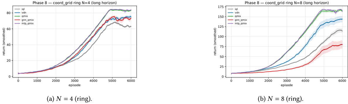
Fig. 7. Phase 8 training curves ( n=10 seeds, 150,000 steps). MLP-QMIX (the parameter-matched no-graph control) tracks QMIX at both scales, while GNN-QMIX is both lower and visibly more variable across seeds: the destabilisation of Finding 3.
