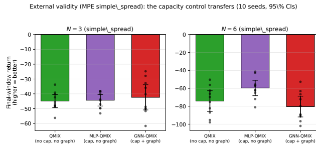
Fig. 4. External validity on MPE simple_spread (10 seeds, 95% CIs; less negative is better). At N=6 , MLP-QMIX (matched parameters, no graph) sits above QMIX while GNN-QMIX falls below both: the positive capacity effect and the negative graph effect the decomposition (Table 6) separates.
