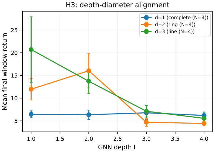
Fig. 11. Phase 4 depth–diameter curves (companion to the heatmap in Section 6.4). Final-window return vs. GCN depth L for each graph diameter d ; the over-depth cliff at L \geq 3 is visible on every diameter.
