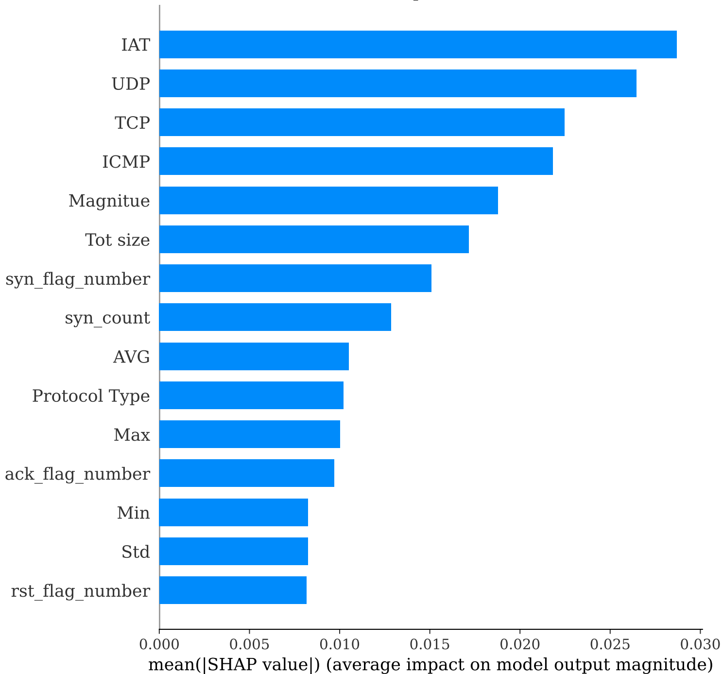
SHAP Global Feature Importance: 1D-CNN (19-class)
