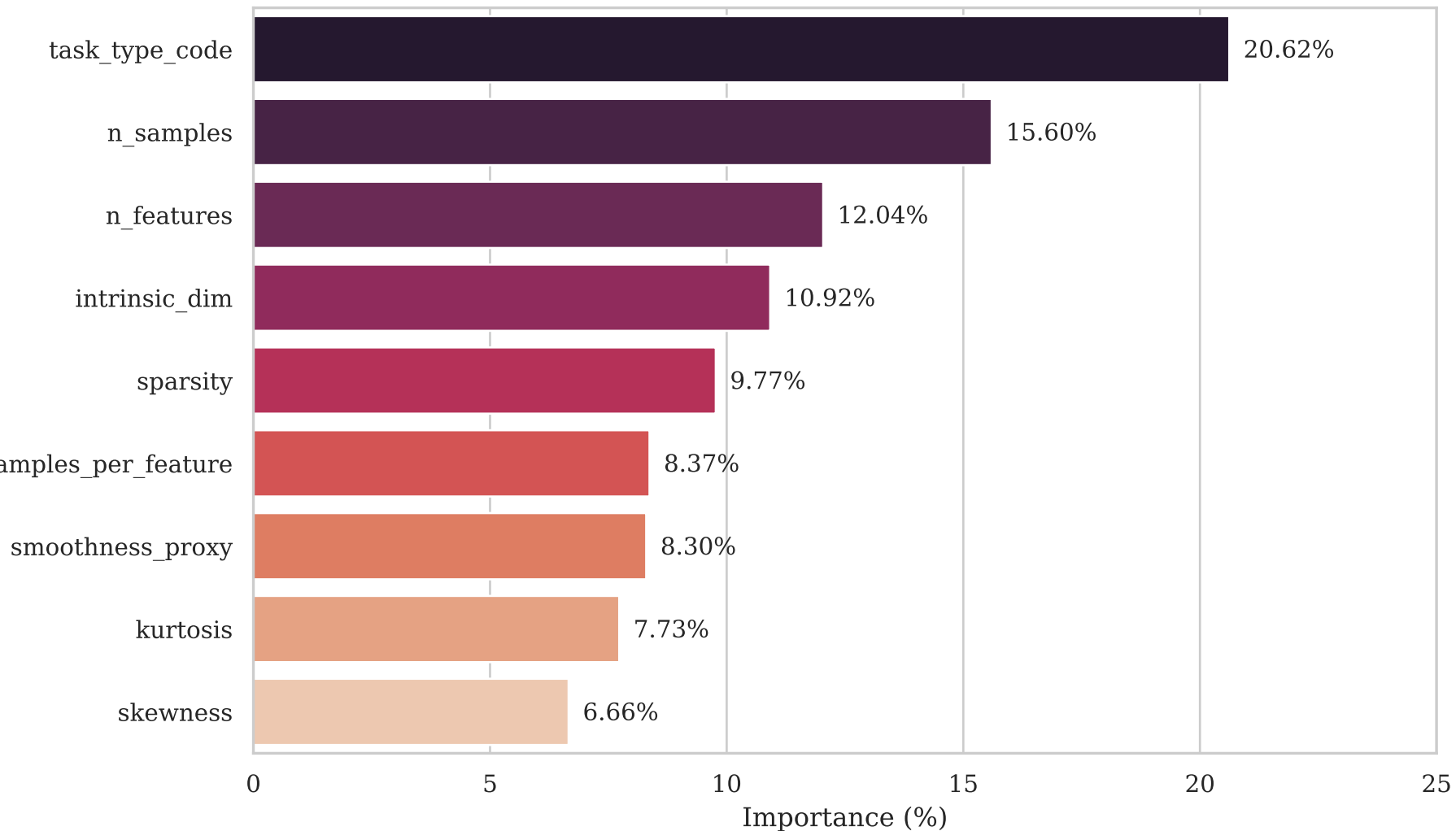
XGBoost Diagnoser: Feature Importance
