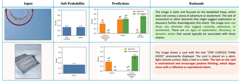
[Manuscript Fig. 5] Qualitative case study on representative Intentionomy samples. Top: the baseline predicts an incorrect alternative and FDIL rejects that distractor using counterfactual rationale evidence. Bottom: a genuine failure of FDIL, on a label with only 0.33 annotator agreement, where its alternative remains semantically plausible.
