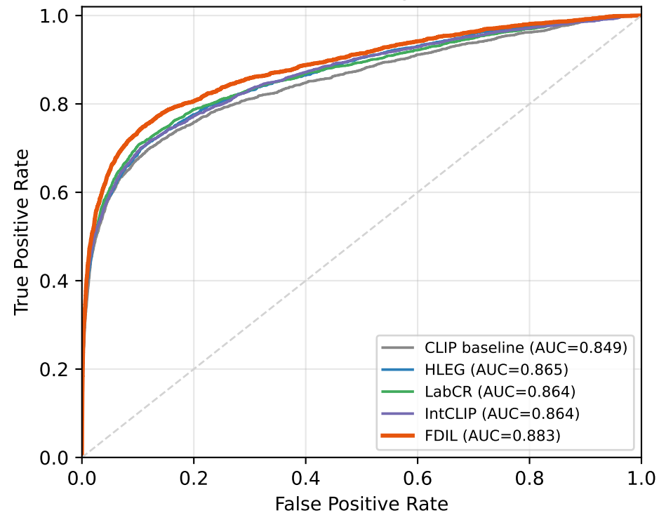
(a) Micro-averaged ROC
