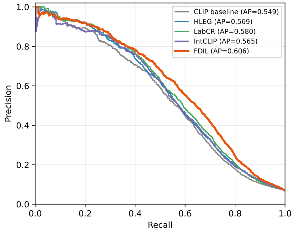
(b) Micro-averaged Precision-Recall
