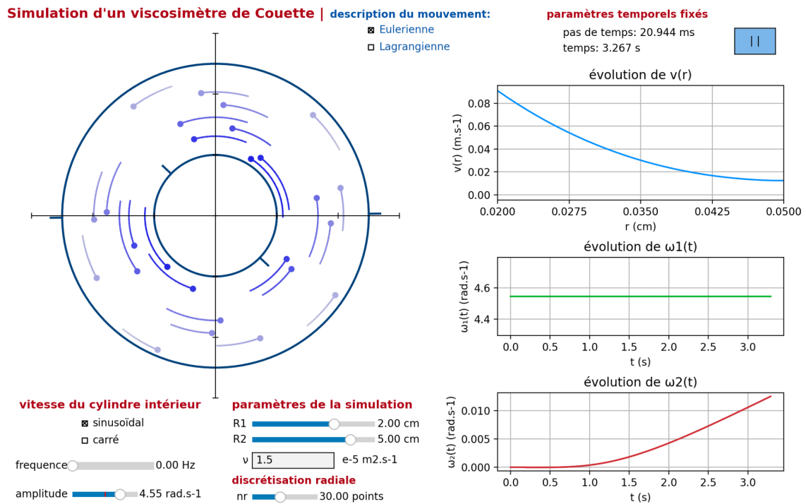
Figure 2: Final user interface of the Couette viscometer simulation. Left: animated cross-section (Eulerian mode shown). Right: live plots of v(r) , \omega_1(t) , and \omega_2(t) . Bottom: interactive parameter controls.
