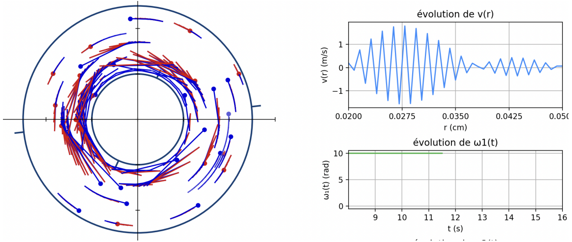
Figure 1: Unstable Explicit Euler Scheme
