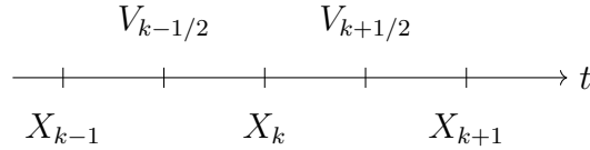
Figure 12: Time diagram of the Leapfrog Verlet method. Positions X_k are evaluated at integer steps, velocities V_{k\pm 1/2} at half-integer steps.
