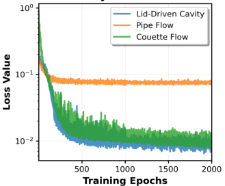
Boundary Condition Loss
