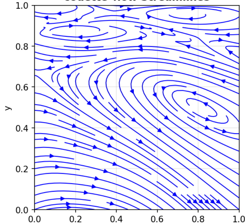
couette flow Streamlines
