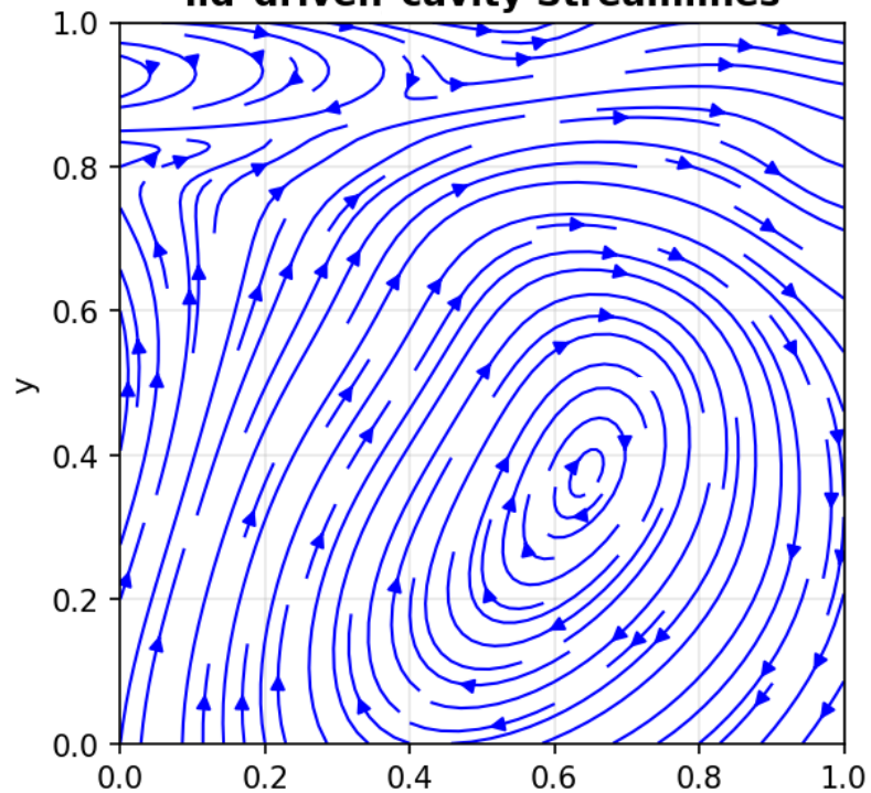
lid driven cavity Streamlines
