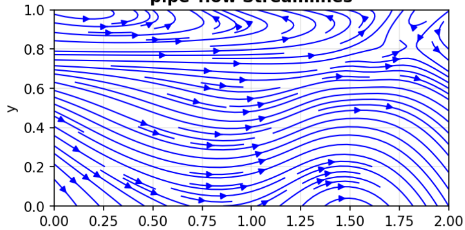
pipe flow Streamlines
