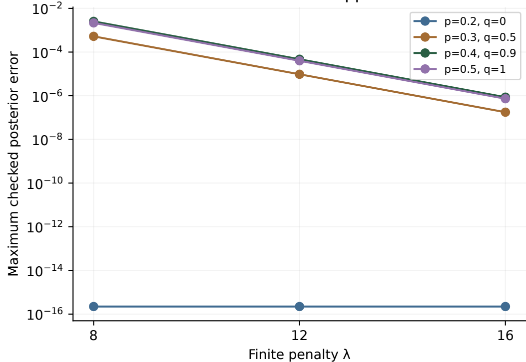
Kac-Ward softened support: L=3
