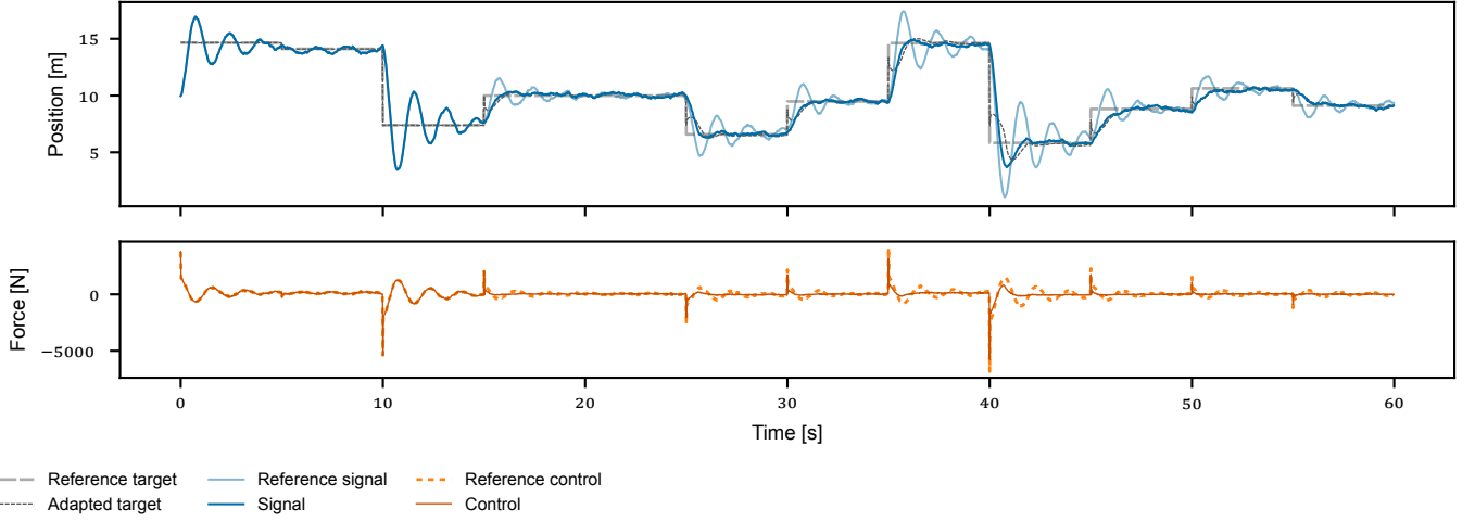
Figure 4: The full minute simulation of the toy problem with an aggressive controller. Top: The system response x and target x_d + \Delta of the adapted controller, alongside the response and target of the unadapted reference controller ( \Delta = 0 ). Bottom: The resulting adapted control inputs from the controller receiving x_d + \Delta alongside the unaltered reference control inputs. During the first 15 seconds (3 targets) the adapter has not received updates yet, and the signal is thus identical to the reference signal.
