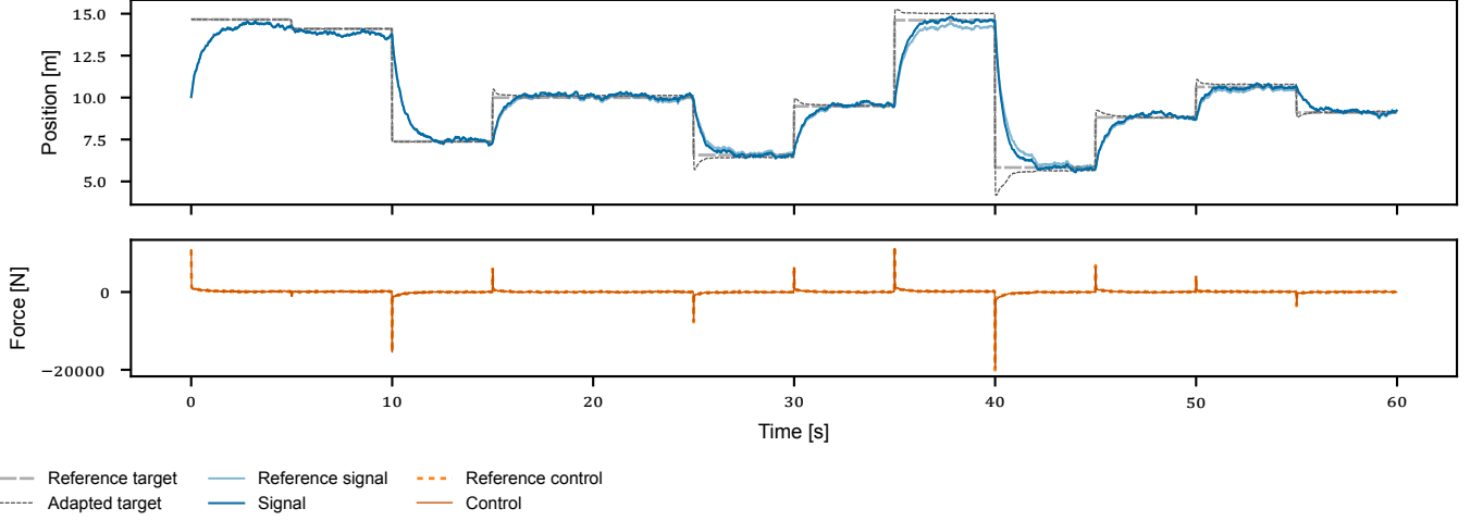
Figure 6: The full minute simulation of the system with an under-responsive controller. Top: The system response and target of the adapted controller, alongside the response and target of the unadapted reference controller. Bottom: The resulting adapted control inputs from the controller receiving the altered target alongside the unaltered reference control inputs.
