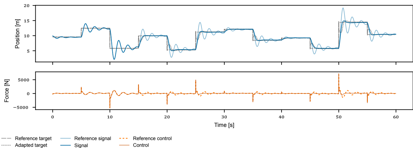
Figure 4: The full minute simulation of the toy problem with an aggressive controller. Top: The system response x and target x_d + \Delta of the adapted controller, alongside the response and target of the unadapted reference controller ( \Delta = 0 ). Bottom: The resulting adapted control inputs from the controller receiving x_d + \Delta alongside the unaltered reference control inputs. During the first 15 seconds (3 targets) the adapter has not received updates yet, and the signal is thus identical to the reference signal.
