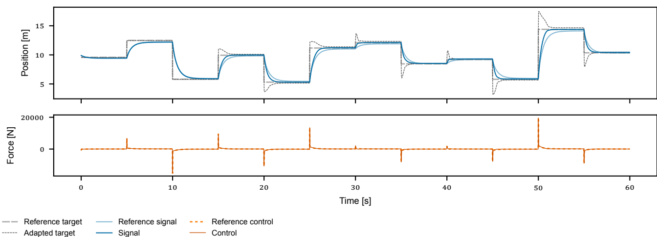
Figure 6: The full minute simulation of the system with an unresponsive controller. Top: The system response and target of the adapted controller, alongside the response and target of the unadapted reference controller. Bottom: The resulting adapted control inputs from the controller receiving the altered target alongside the unaltered reference control inputs.
