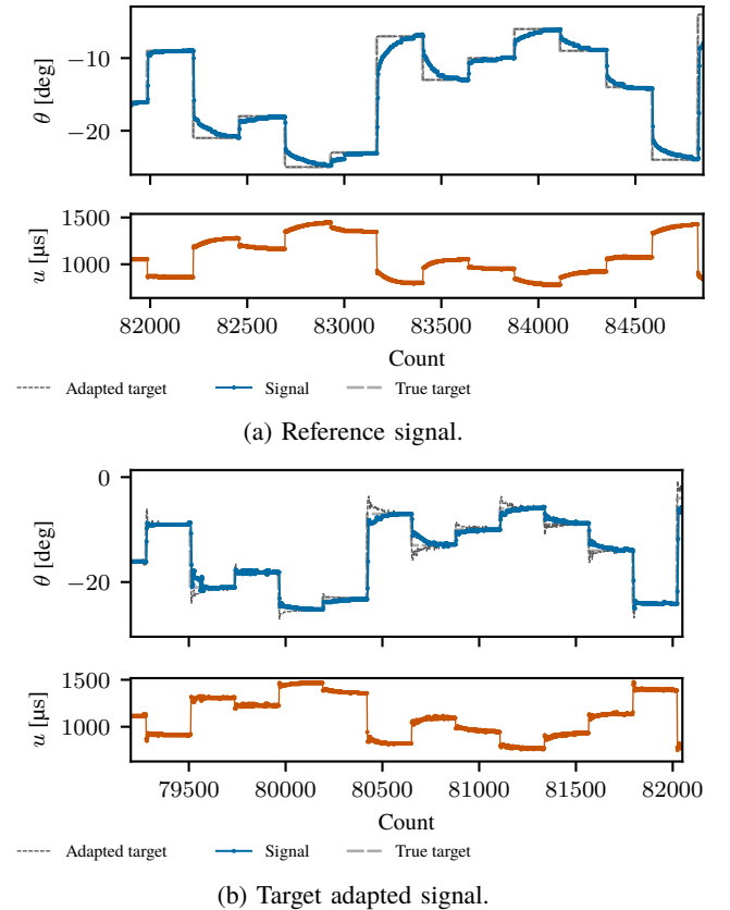
Fig. 15: Qualitative comparison of 1min of the signal response for the under-tuned PID controller.
