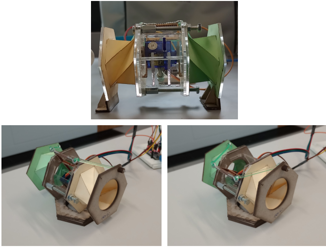
Fig. 12: Top : The “feet” of the robot grip when dragged backwards, but slide when pushed forward, allowing the robot to move forward, also known as two-anchor crawling (Calisti et al., 2017). Left : The robot at its fully extended state, corresponding to the “home” position of the servo and actuation arm. Right : The fully contracted robot, corresponding to the maximum (capped) servo output, near the mechanical limit of the actuation arm.
