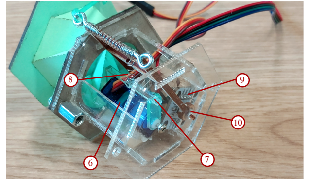
(a) The Kresling origami robot.
