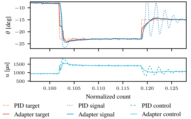
Fig. 23: A close-up from the slow-aggressive PID controller with target adapter. The manner in which the target is adapted resembles that of Figure 6 from the toy problem.
