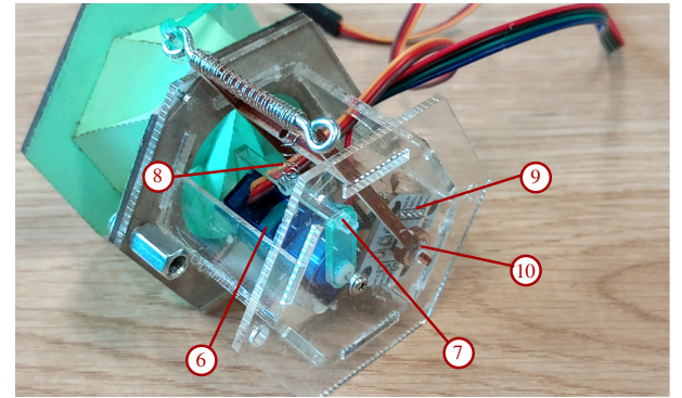
(a) The Kresling origami robot.
