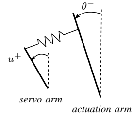
Fig. 12: Nominal signs of the angles for the servo and actuation arm during operation.
