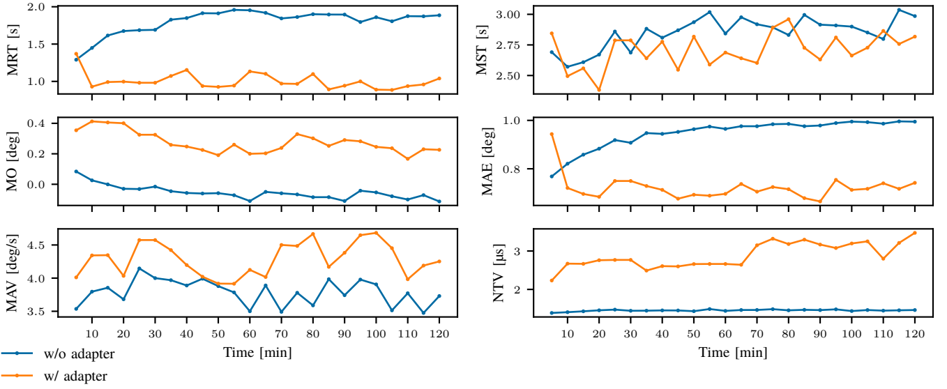
Fig. 16: Metrics evolution over the duration of the experiment for an under-tuned PID controller. Each point represents the calculated value of the metric on identical 5min sequences of targets. Plots for all metrics and numerical values can be found in Figure B.2 and Table B.II, respectively.
