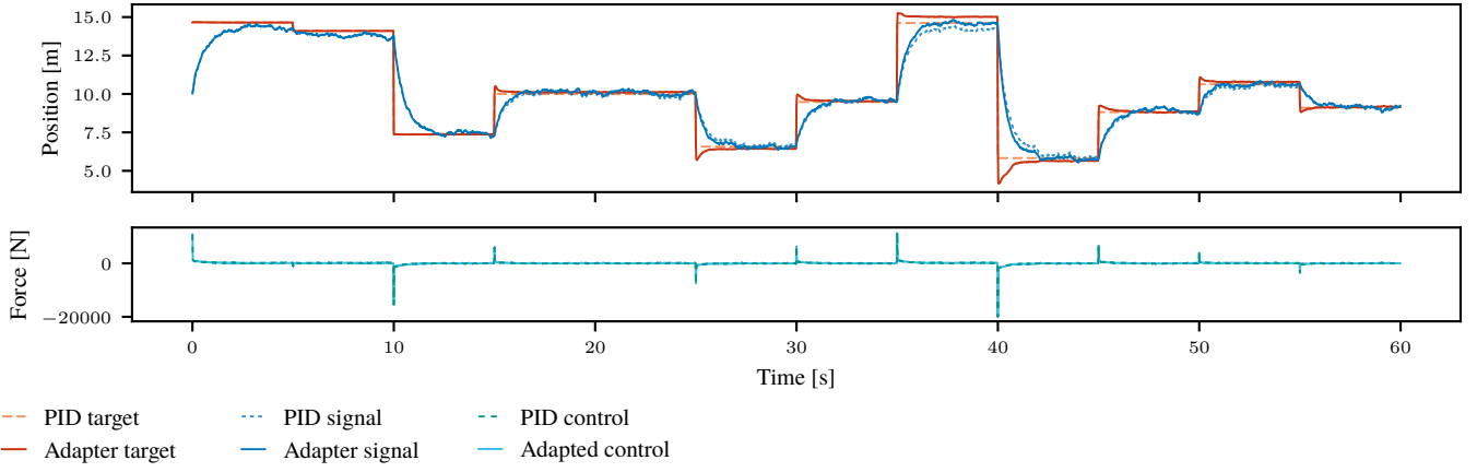
Fig. 7: The full minute simulation of the system with an under-responsive controller. Top : The system response and target of the adapted controller, alongside the response and target of the unadapted reference controller. Bottom : The resulting adapted control inputs from the controller receiving the altered target alongside the unaltered reference control inputs.
