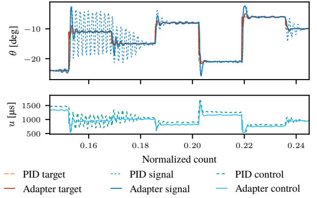
Fig. 13: Qualitative comparison between the behavior of the baseline controller and target adapted controller for the slow-aggressive PID controller.
