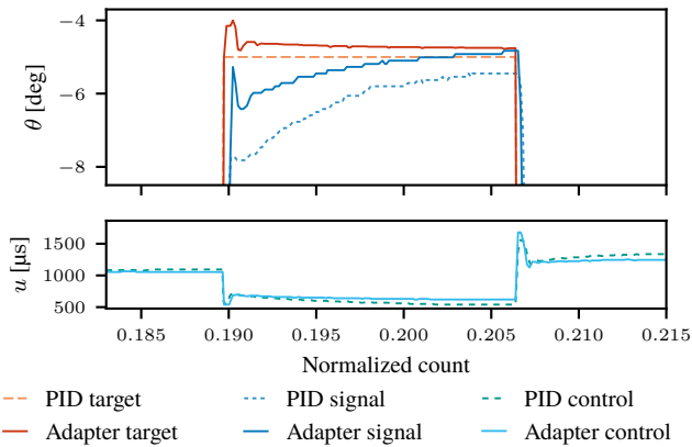
Fig. 22: A close-up from the 0.5–0.5mm perforation with target adapter. The signal response generally resembles that of Figure 8 from the toy problem.
