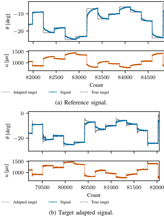
Fig. 14: Qualitative comparison of 1min of the signal response for the under-tuned PID controller.
