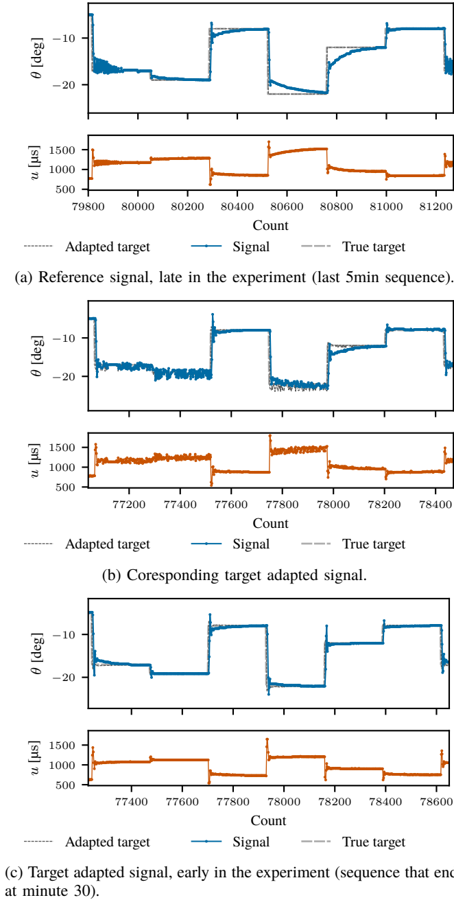
Fig. 18: Qualitative comparison of 30s of the signal response for the 2-0.5mm perforation. Also showing a comparison between the signals of the target adapted controller, late vs. early into the experiment.
