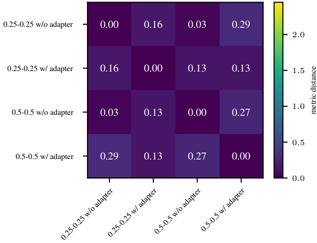
Fig. D.3: Distance in the metric space between the KOSs at the start of the 0.25–0.25mm and 0.5–0.5mm perforation experiment.
