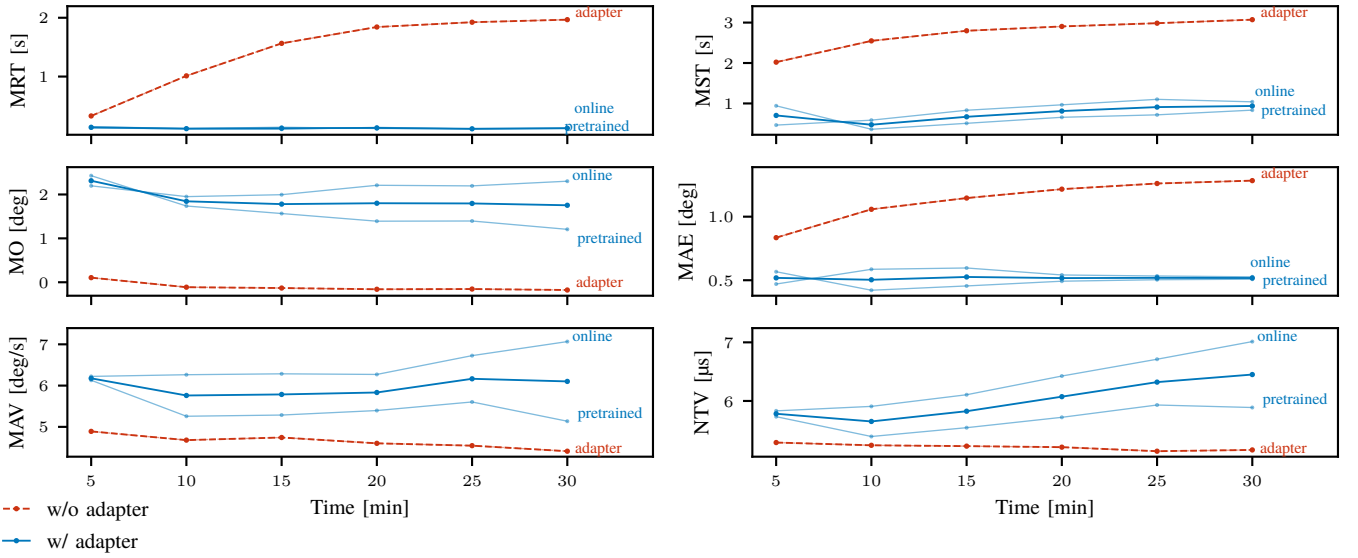
Fig. C.5: Metrics evolution for the crawling gait experiment.
