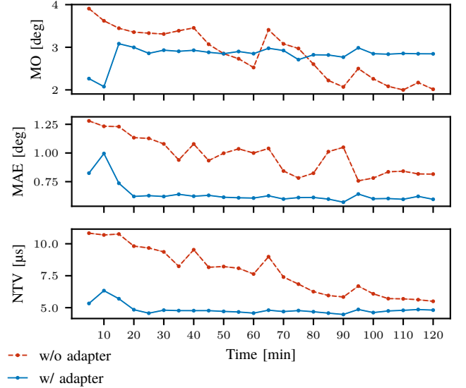
Fig. 16: Metrics evolution over the 2h duration of the experiment for an aggressive but under-responsive PID controller. Each point represents the calculated value of the metric on identical 5min sequences of targets. Plots for all metrics and numerical values can be found in Figure C.1 and Table C.I, respectively.
