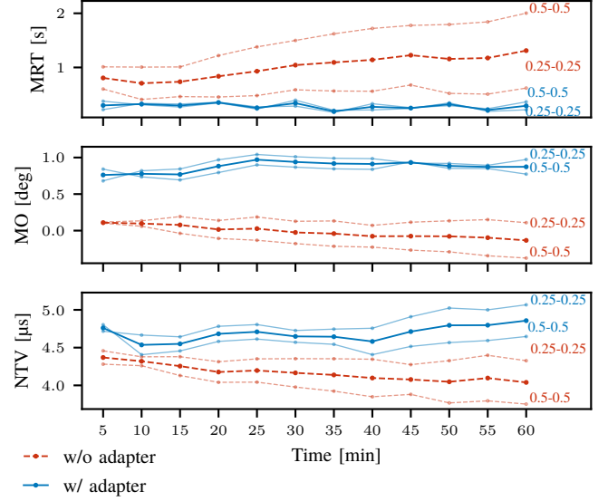
Fig. 19: Metrics evolution over the 1h duration of the experiment for KOSs in a lower state of degradation (0.25–0.25mm and 0.5–0.5mm perforations, see annotations), with their average overlaid. Each point represents the calculated value of the metric on identical 5min sequences of targets. Plots for all metrics and numerical values can be found in Figure C.3 and Table C.III, respectively.
