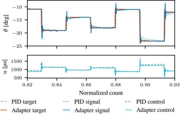
(b) A comparison early in the experiment (5min sequence that ends at minute 30).
