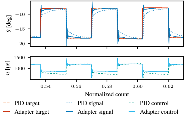
Fig. 23: Qualitative comparison between the behavior of the baseline controller and target adapted controller for the crawling gait experiment.
