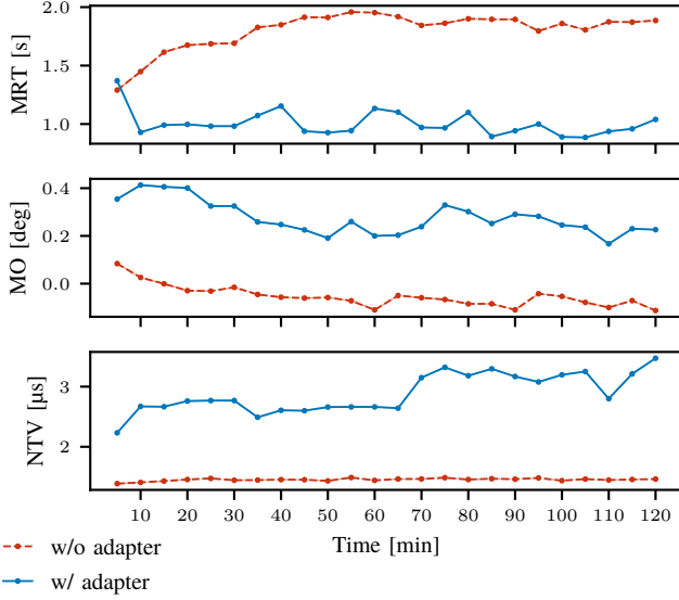
Fig. 17: Metrics evolution over the duration of the experiment for an under-tuned PID controller. Each point represents the calculated value of the metric on identical 5min sequences of targets. Plots for all metrics and numerical values can be found in Figure C.2 and Table C.II, respectively.
