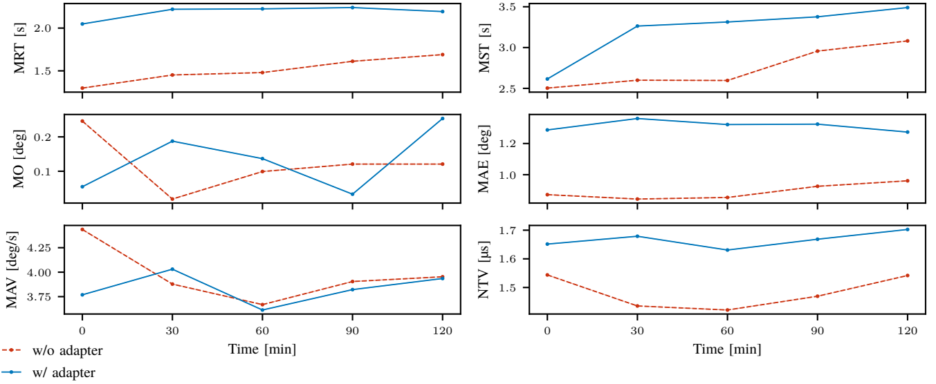
Fig. D.7: Reference minute metrics evolution of the under-tuned PID experiment.
