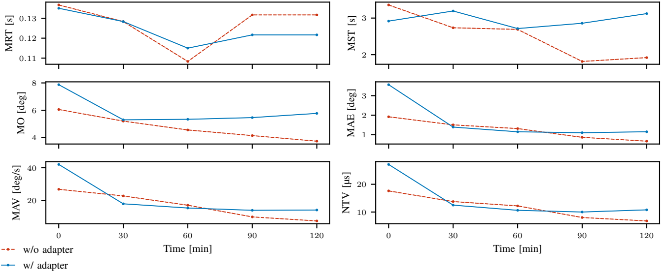
Fig. D.6: Reference minute metrics evolution of the slow-aggressive PID experiment.
