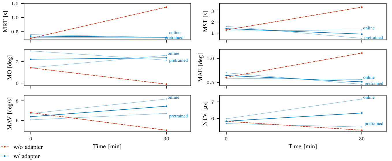
Fig. D.9: Reference minute metrics evolution of the crawling gait experiment.
