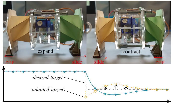
Fig. 1: The Kresling-origami robot with target adaptation. Top : The “feet” of the robot grip when dragged backwards, but slide when pushed forward, allowing the robot to move forward, also known as two-anchor crawling (Calisti et al., 2017). Bottom : The contraction target is adapted to reduce overshoot and unstable oscillations.
