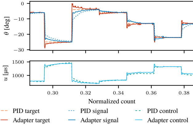
Fig. 18: Qualitative comparison between the behavior of the baseline controller and target adapted controller for the under-tuned PID controller.
