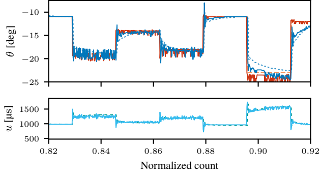
(a) A comparison late in the experiment (last 5min sequence).
