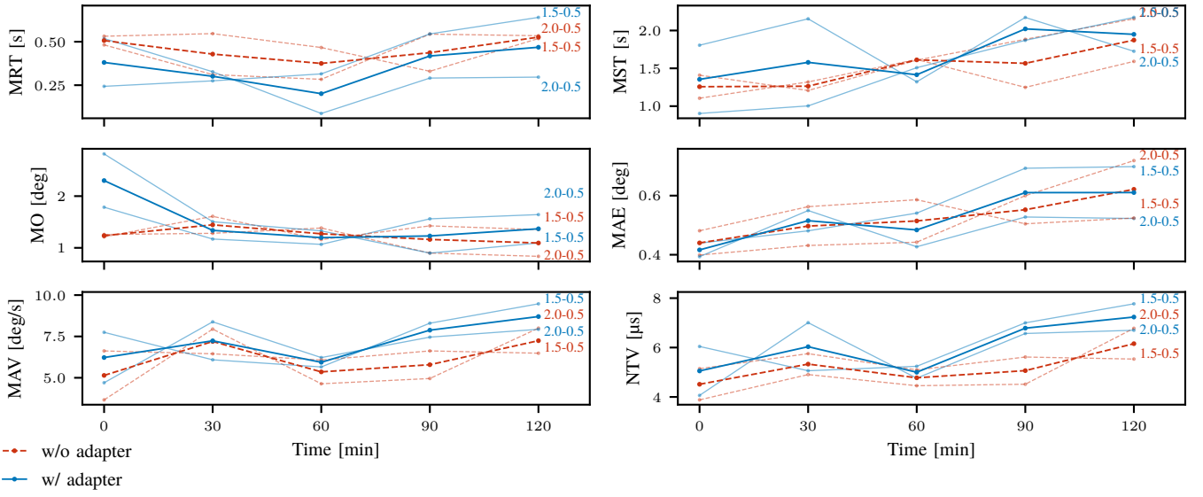
Fig. D.8: Reference minute metrics evolution of the 1.5–0.5mm and 2–0.5mm perforation experiment.
