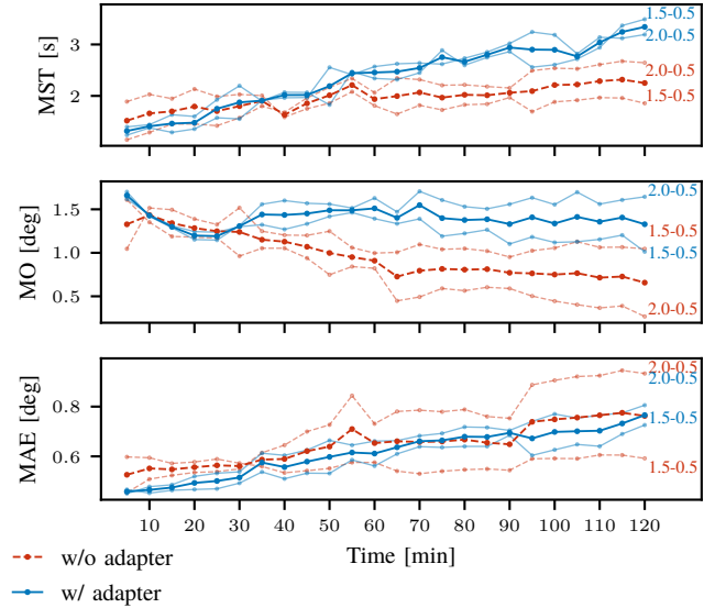
Fig. 20: Metrics evolution over the 2h duration of the experiment for KOSs in a higher state of degradation (1.5–0.5mm and 2–0.5mm perforations, see annotations), with their average overlaid. Each point represents the calculated value of the metric on identical 5min sequences of targets. Plots for all metrics and numerical values can be found in Figure C.4 and Table C.IV, respectively.
