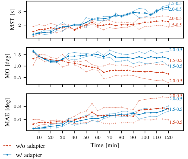
Fig. 20: Metrics evolution over the 2h duration of the experiment for KOSs in a higher state of degradation (1.5–0.5mm and 2–0.5mm perforations, see annotations), with their average overlaid. Each point represents the calculated value of the metric on identical 5min sequences of targets. Plots for all metrics and numerical values can be found in Figure B.4 and Table B.IV, respectively.
