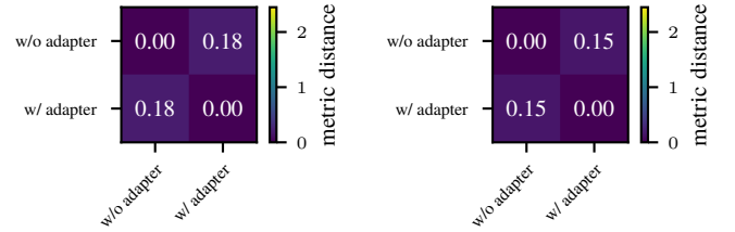
(a) Distance in the metric space between the KOSs at the start of the slow-aggressive PID experiment. (b) Distance in the metric space between the KOSs at the start of the under-tuned PID experiment.
