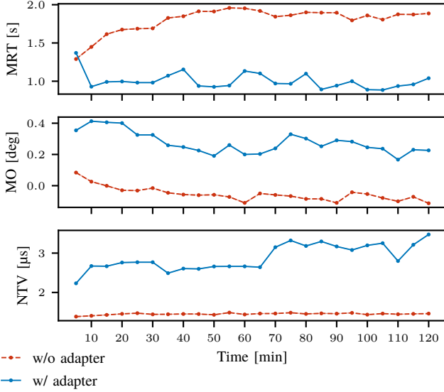
Fig. 18: Metrics evolution over the duration of the experiment for the under-tuned PID controller. Each point represents the calculated value of the metric on identical 5min sequences of targets. Plots for all metrics and numerical values can be found in Figure C.2 and Table C.II, respectively.
