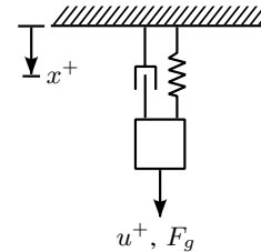
Fig. 4: Setup of the mass-spring-damper system in the toy problem with positive directions indicated.
