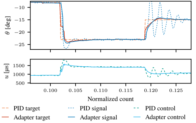
Fig. 25: A close-up from the slow-aggressive PID controller with target adapter. The manner in which the target is adapted resembles that of Figure 8 from the toy problem.
