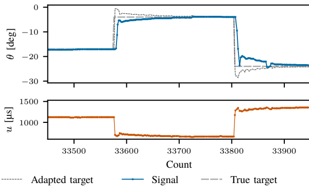
Fig. 22: A close-up from the under-tuned PID controller with target adapter. The signal response generally resembles that of Figure 8 from the toy problem.
