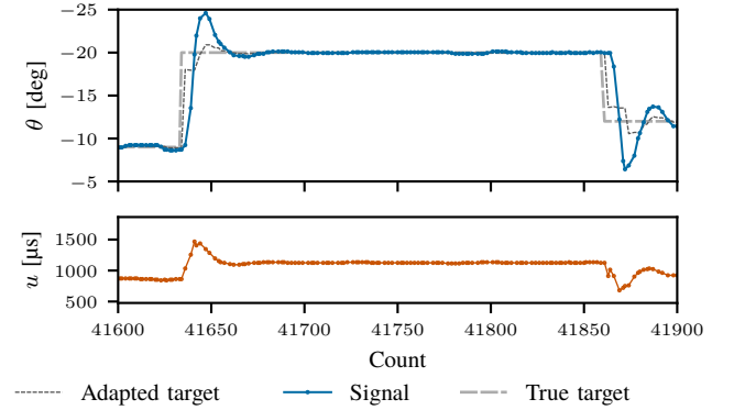
Fig. 23: A close-up from the slow-aggressive PID controller with target adapter. The manner in which the target is adapted resembles that of Figure 6 from the toy problem.
