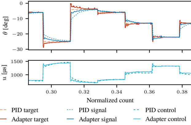
Fig. 17: Qualitative comparison between the behavior of the baseline controller and target adapted controller for the under-tuned PID controller.
