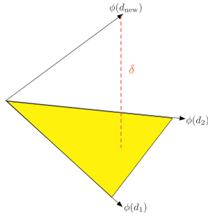
(a) “Geometrical interpretation of the independence measure \delta . Here, the dictionary consists of two data points \{d_1, d_2\} which span a linear plane in the feature space. The independence measure \delta for a new data point d_{new} can be interpreted as the distance to this plane.” (Nguyen-Tuong & Peters, 2011a). Figure and caption obtained from Nguyen-Tuong and Peters (2011a).
