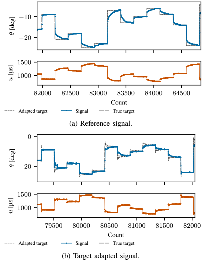
Fig. 15: Qualitative comparison of 1min of the signal response for the under-tuned PID controller.
