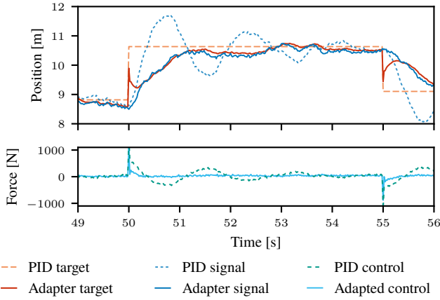
Fig. 6: A close-up of the second to last target in the one-minute simulation. The effects of the adapter can be more clearly observed: The overshoot (seen in the reference signal) is countered by bringing the target closer to the current state.
