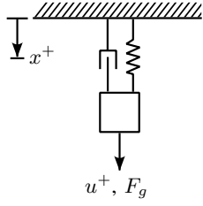
Fig. 4: Setup of the mass-spring-damper system in the toy problem with positive directions indicated.
