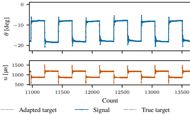
(b) Target adapted signal for the fully online trained adapter.
