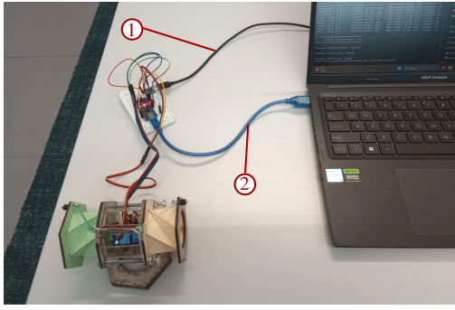
Fig. 11: The test setup.
