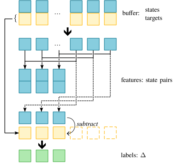
(b) The feature and label extraction process: recorded states spaced by a specified prediction window are paired up and provided as features to the adapter, which learns to predict a \Delta , being the difference between the target \mathbf{x}_{d,t} and state \mathbf{x}_{t+window} .
