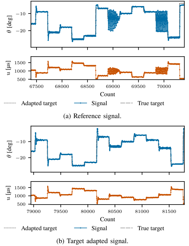
Fig. 13: Qualitative comparison of 1min of the signal response for the slow-aggressive PID controller.
