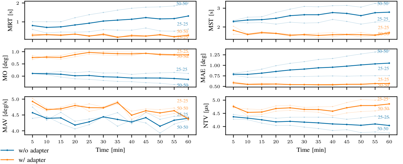
Fig. 17: Metrics evolution over the 1h duration of the experiment for KOSs in a lower state of degradation (0.25–0.25mm and 0.5–0.5mm perforations, see annotations), with their average overlaid. Each point represents the calculated value of the metric on identical 5min sequences of targets. Numerical values can be found in Appendix C.
