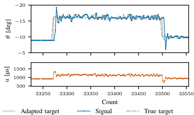
Fig. 24: A close-up of the 2–0.5mm experiment. The oscillations in the signal response are recorded at an insufficient frequency to contain any meaningful relationship between spaced-out state pairs and the target. As a result, the adapter's output becomes more chaotic as well, further polluting the training data.
