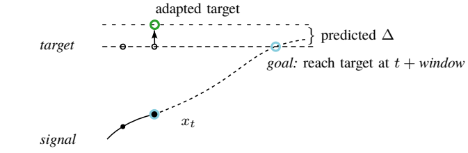
(a) By supplying the model with the controller's target position and current state x_t it yields a \Delta that can be added to the current target, which will supposedly result in the controller reaching the target within the specified window.
