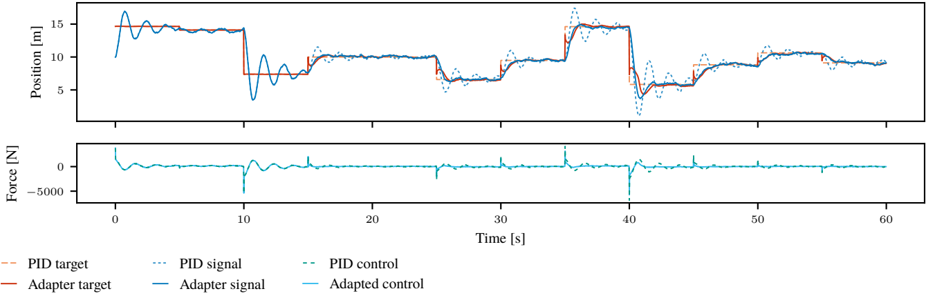
Fig. 5: The full minute simulation of the toy problem with an aggressive controller. Top: The system response x and target x_d + \Delta of the adapted controller, alongside the response and target of the unadapted reference controller ( \Delta = 0 ). Bottom: The resulting adapted control inputs from the controller receiving x_d + \Delta alongside the unaltered reference control inputs. During the first 15s (3 targets) the adapter has not received updates yet, and the signal is thus identical to the reference signal.
