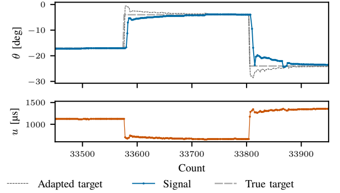
Fig. 22: A close-up from the under-tuned PID controller with target adapter. The signal response generally resembles that of Figure 8 from the toy problem.
