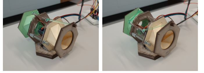
Fig. 10: Left : The robot at its fully extended state, corresponding to the “home” position of the servo and actuation arm. Right : The fully contracted robot, corresponding to the maximum (capped) servo output, near the mechanical limit of the actuation arm.
